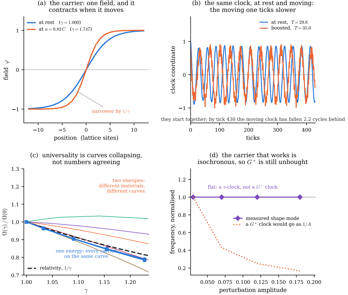
Figure 11: The carrier arc, watched rather than tabulated. (a) The carrier itself: one field, whose profile contracts by 1/\gamma when it moves. (b) The claim, directly. The internal clock's trace at rest and boosted, released in phase: the moving clock has fallen 2.2 cycles behind by tick 430. The roughness on the boosted trace is real — a boosted lattice kink radiates. (c) Universality as convergence. Two-category carriers fan apart, one of them running faster when moving; at \gamma = 1.22 they span 0.283 while the one-energy carriers span 0.006, a factor of 46. The one-energy curves collapse onto each other and lie a little below 1/\gamma , the residual discussed in the text. (d) Why this is still not the G^* clock: the shape-mode frequency is flat in amplitude — isochronous to \leq 0.23\% , set by the FFT bin — where a quartic clock would fall as 1/A .
