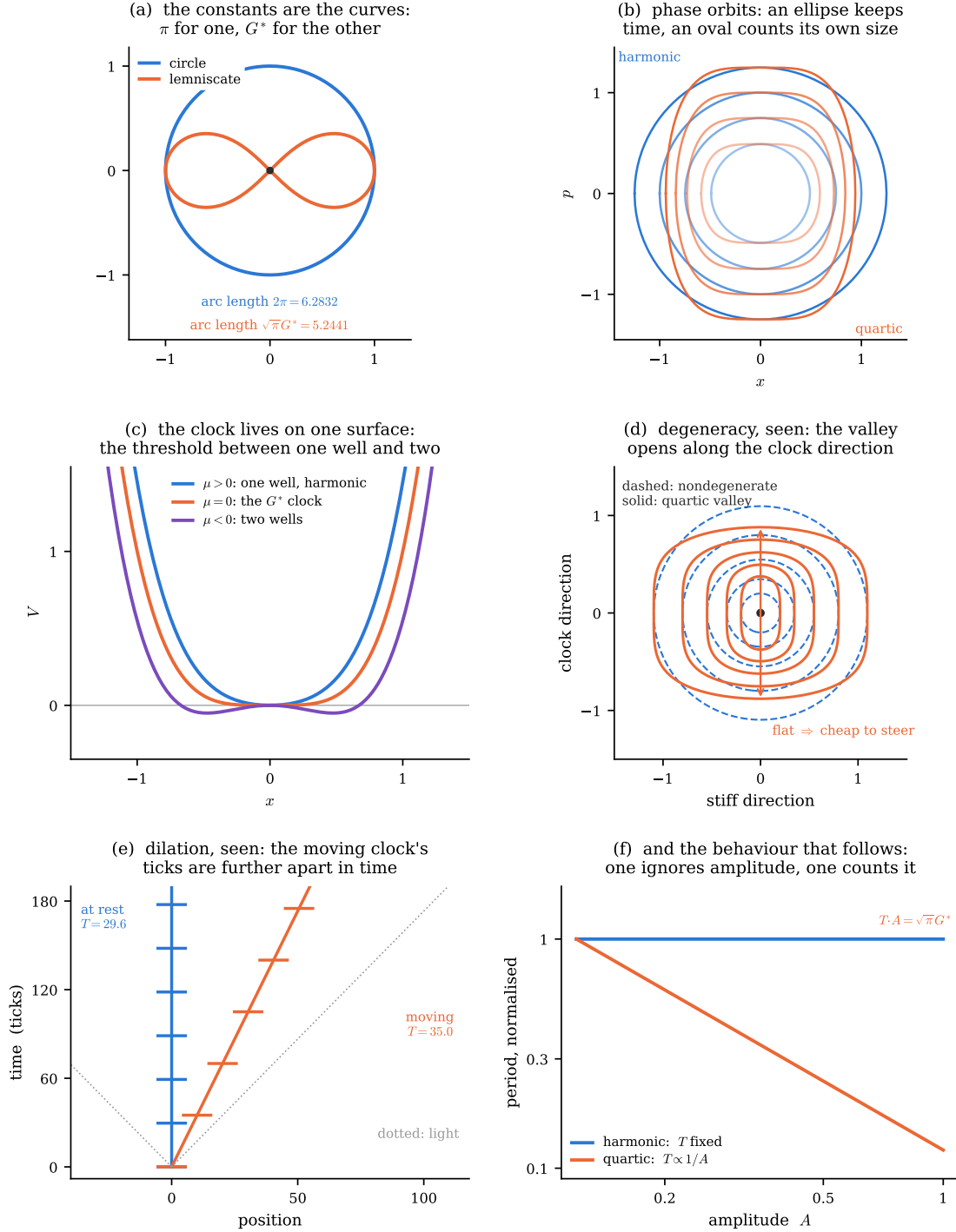
Figure 12: The two clocks, seen. (a) The constants are not normalisations but arc lengths: the unit circle's is 2\pi = 6.2832 , the unit lemniscate's is \sqrt{\pi}G^* = 5.2441 — the latter integrated numerically here and agreeing with B(\frac{1}{4}, \frac{1}{2}) to 10^{-7} . (b) Phase orbits at equal energy steps: harmonic level sets are ellipses traversed uniformly, so the period ignores the orbit's size; quartic ones are flat-flanked ovals and are traversed faster as they grow. (c) The degenerate clock does not live at a generic point but on a single surface — the threshold \mu = 0 between one well and two, where the cubic is forbidden by symmetry and the quartic is what remains. (d) The degeneracy made visible: contours about a nondegenerate minimum are closed ellipses (dashed), while the quartic valley (solid) opens along the clock direction. That flatness is the cheapness of (25). (e) Dilation as geometry, drawn from the measured kink periods: tick events on two worldlines, one at rest and one at u = 0.5C , with the moving clock's ticks further apart in time. (f) The behaviour that follows.
