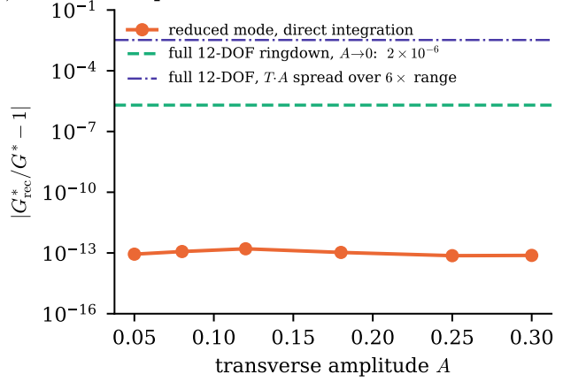
Figure 3: The minimum viable clock carrier. (a) Four bodies, three unit bonds carrying tension and one single-bond strut at range 3r_0 carrying compression; the self-stress is \omega = (1, 1, 1, -1) and the blocking form is positive definite on every nontrivial flex, so the object is prestress-stable at zero tension. (b) The period law (14) verified without a fitted scale: direct integration of the reduced mode reproduces it to machine precision, and the two horizontal lines mark the independent full twelve-degree-of-freedom result.
