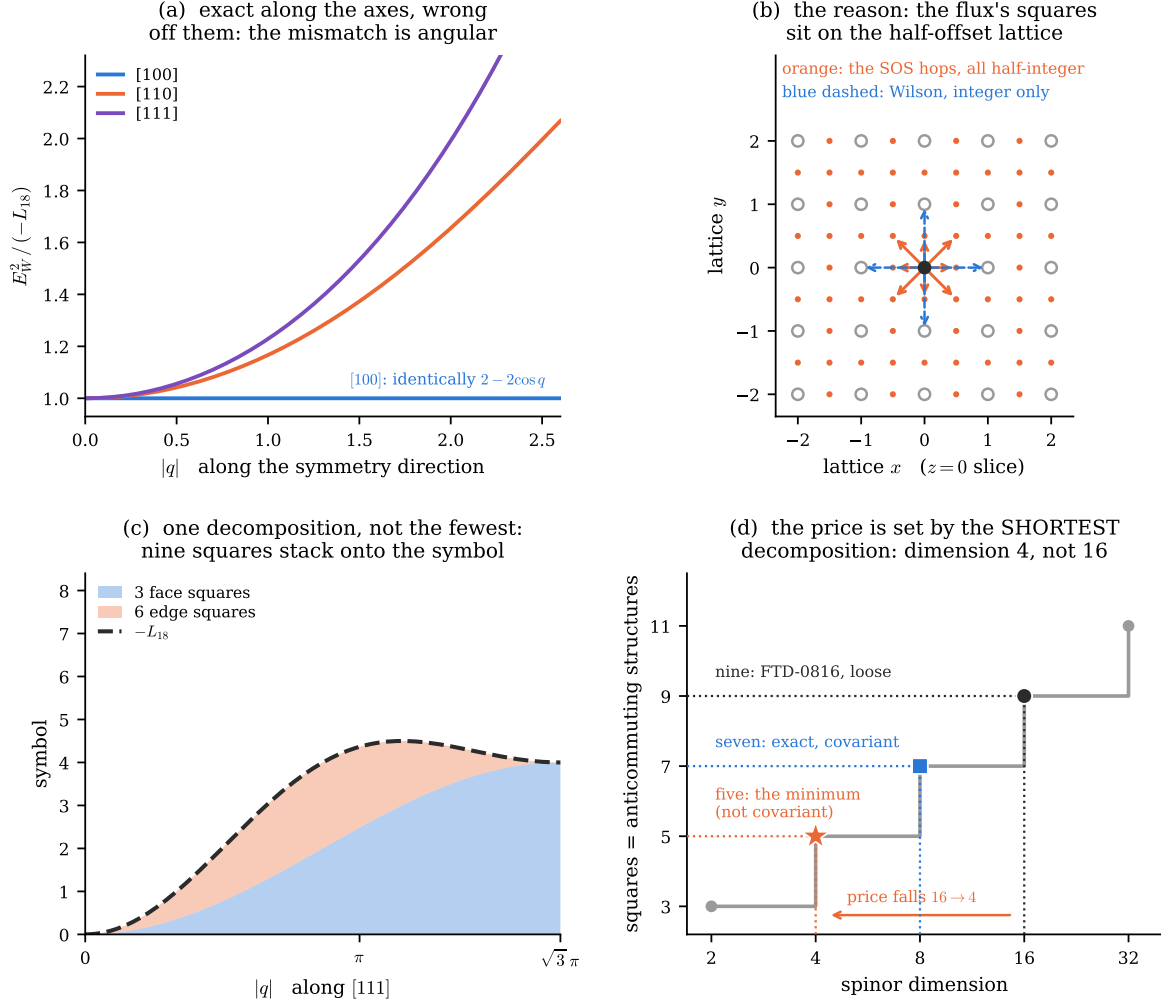
Figure 10: Why two sectors miss, and what a hit costs. (a) Normalised to a common slope, the flux symbol and a Wilson operator agree identically along the cubic axes — both are 2 - 2 \cos q — and diverge only off them, reaching 1.65 along [110] and 1.99 along [111] at |q| = 2 . The mismatch is purely angular, so no rescaling is even the right shape. (b) The reason, in the z = 0 slice: the flux symbol's nine squares carry arguments q_i/2 and (q_i \pm q_j)/2 , i.e. hops of half a lattice unit (orange), while Wilson hops land on integer sites (blue dashed). The sectors were being matched on different lattices. (c) One such identity: three face squares and six edge squares stack exactly onto -L_{18} , with residual 1.8 \times 10^{-15} over 4000 random momenta. (d) The price, which is set by the shortest decomposition rather than by any one of them. n squares require n mutually anticommuting structures and dimension 2^k carries 2k + 1 , so nine would cost spinor dimension 16; but nine is not the fewest. An exact cubic-covariant seven -square identity holds, -L_{18} = 4 \sum_i \sin^2 x_i \cos^2 x_j \cos^2 x_k + \frac{16}{3} \sum_i \sin^2 x_j \sin^2 x_k \cos^2 x_i + 4 \sin^2 x_1 \sin^2 x_2 \sin^2 x_3 with x = q/2 , costing dimension 8; and a search over the nearest-neighbour class finds a five at dimension 4 — ordinary Dirac — which is genuinely non-covariant. The fourfold taste multiplication was an artefact of a non-minimal decomposition, not a feature of the symbol.
