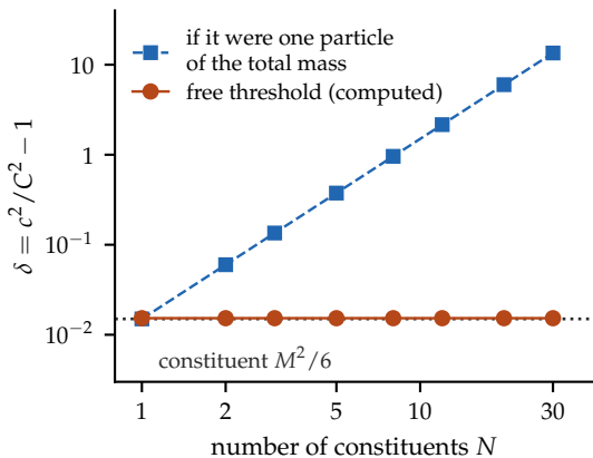
(c) free N -particle threshold cone shift is N -independent (not a bound state)
