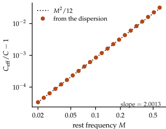
(a) the limiting speed depends on the rest mass, as M^2/12
