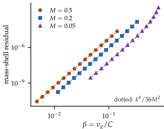
(b) the free mass-shell diagnostic has a known O(\beta^4) residual
