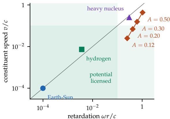
(d) the clock sits outside both limits its own model assumes
