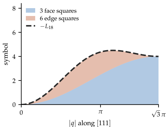
(c) one decomposition, not the fewest: nine squares stack onto the symbol
