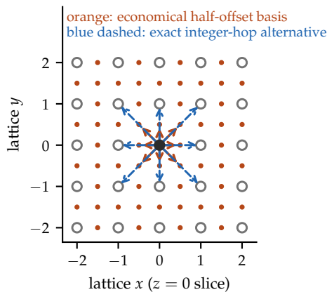
(b) two exact placement classes: half-offset economy, integer-hop existence
