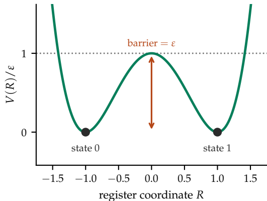
(d) register: two states, one barrier, and it is the same \epsilon
