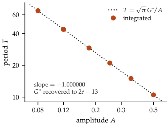
(c) ideal normal-form clock law, no fitted scale: slope -1 and the constant is G^*
