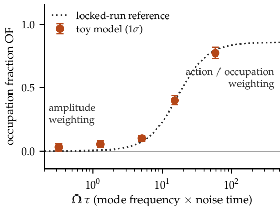
(f) gate: the classical threshold statistic interpolates with the timescale ratio
