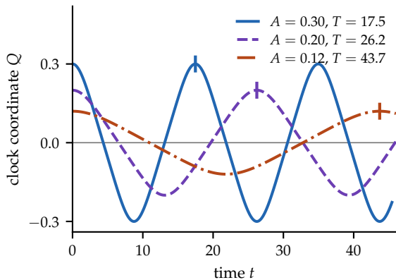
(b) clock: a bigger swing is a faster clock (ticks mark one period)
