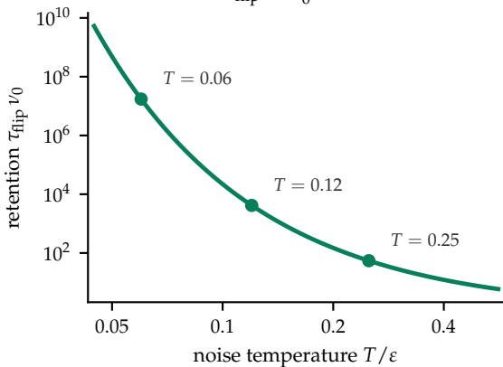
(e) retention is Arrhenius:
