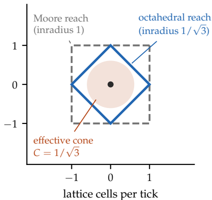
(a) substrate: the effective cone sits inside every candidate causal polytope
