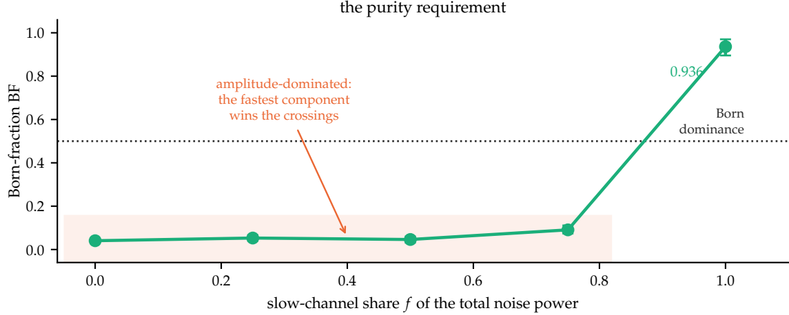
Figure 8: The purity requirement. Mixing a slow channel into fast noise does not gradually produce Born weighting; the statistics remain amplitude-dominated until the slow channel is nearly exclusive.
