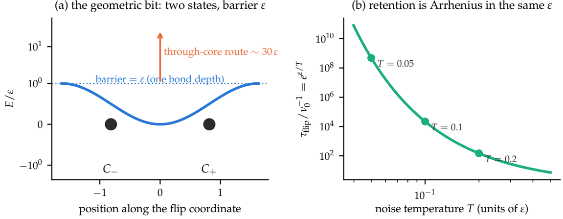
Figure 5: The geometric bit. (a) Two mirror states separated by a barrier of exactly one bond depth along the hinge path; the direct route through the repulsive core costs about thirty times as much, and a watershed over the full configuration space confirms no cheaper channel exists. (b) The same \epsilon fixes retention through an Arrhenius law, so the memory’s lifetime is set by the constant that binds the matter.
