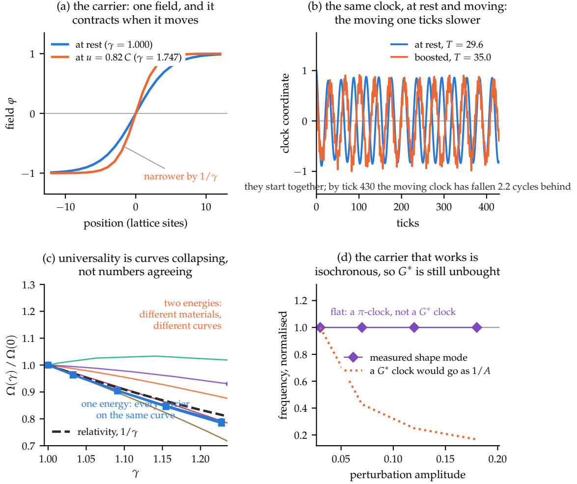
Figure 12: The carrier arc, watched rather than tabulated. (a) The carrier itself: one field, whose profile contracts by 1/\gamma when it moves. (b) The claim, directly. The internal clock's trace at rest and boosted, released in phase: the moving clock has fallen 2.2 cycles behind by tick 430. The roughness on the boosted trace is real — a boosted lattice kink radiates. (c) Universality as convergence. Two-category carriers fan apart, one of them running faster when moving; at \gamma = 1.22 they span 0.283 while the one-energy carriers span 0.006, a factor of 46. The one-energy curves collapse onto each other and lie a little below 1/\gamma , the residual discussed in the text. (d) Why this is still not the G^* clock: the shape-mode frequency is flat in amplitude — isochronous to \leq 0.23\% , set by the FFT bin — where a quartic clock would fall as 1/A .
