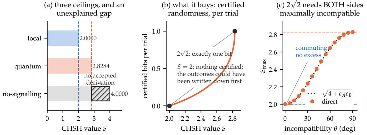
Figure 9: The three ceilings, computed. (a) Local correlations stop at 2, quantum at 2\sqrt{2} , and no-signalling at 4; the hatched band is the 29.3% that relativistic consistency permits and nature does not use. (b) What the number buys: the device-independent min-entropy runs from exactly zero certified bits at S = 2 — where the outcomes could have been written down in advance — to exactly one bit at 2\sqrt{2} . (c) The price, from S^2 = 4 + \|[A_0, A_1]\| \|[B_0, B_1]\| : each commutator norm is capped at 2, so a product of 4 requires both at maximum. There is no partial-credit route to 2\sqrt{2} . The dotted curve is the identity and the markers are the directly computed operator norm; they agree to 2 \times 10^{-15} .
