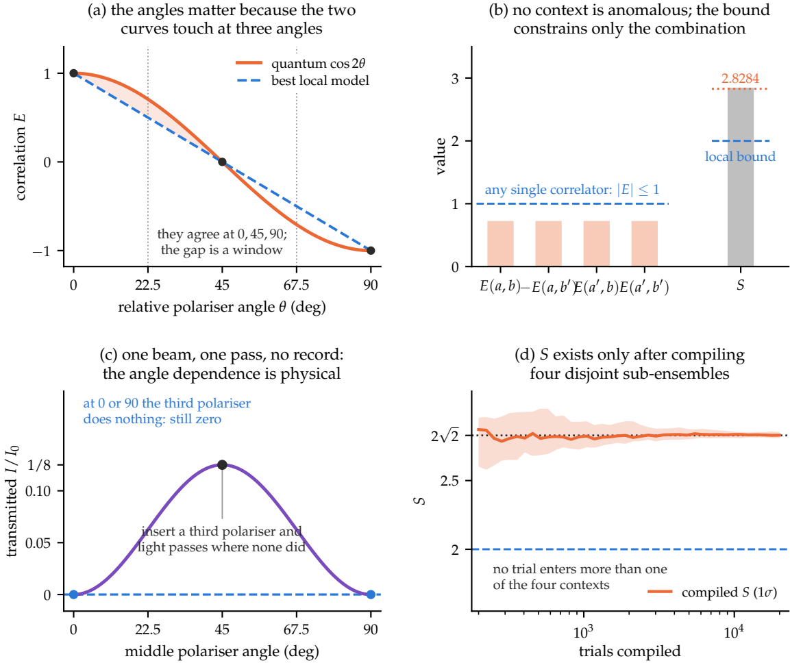
Figure 10: The angles, and the boundary. (a) For polarisation-entangled light the quantum correlation \cos 2\theta and the best local model — a straight line — touch at 0^\circ , 45^\circ and 90^\circ , so the violation is an angle window rather than a uniform excess; the widest single gap is 0.211 at 19.85^\circ . (b) At the CHSH settings each of the four contexts contributes exactly 1/\sqrt{2} , well inside the |E| \leq 1 available to any correlator: no context is individually anomalous, and the local bound constrains only the total. (c) Two crossed polarisers transmit nothing; inserting a third at 45^\circ transmits I_0/8 . One beam, one pass, no ensemble comparison and no record — the angle dependence is physical, not a feature of the bookkeeping. (d) S by contrast is a compiled statistic: the four sub-ensembles are verified disjoint and exhaustive, no trial enters more than one, and the number exists only after all four are combined.
