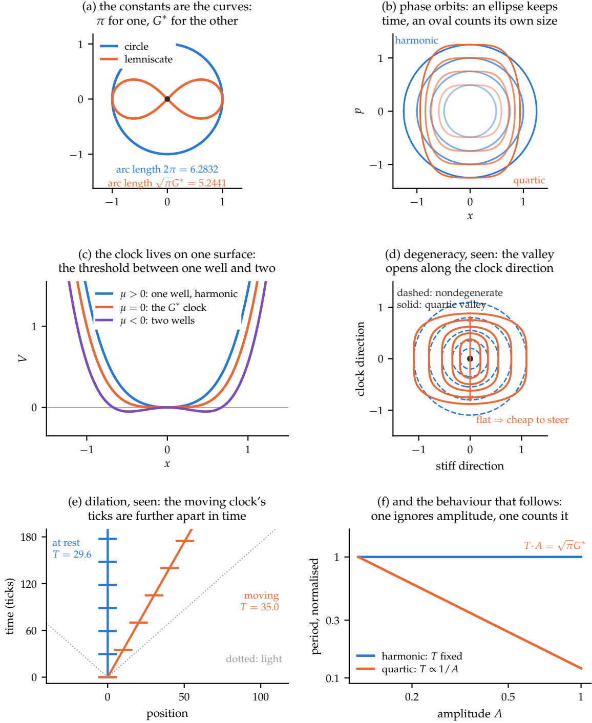
Figure 4: The two clocks, seen. (a) The constants are not normalisations but arc lengths: the unit circle's is 2\pi = 6.2832 , the unit lemniscate's is \sqrt{\pi G^*} = 5.2441 — the latter integrated numerically here and agreeing with B(\frac{1}{4}, \frac{1}{2}) to 10^{-7} . (b) Phase orbits at equal energy steps: harmonic level sets are ellipses traversed uniformly, so the period ignores the orbit's size; quartic ones are flat-flanked ovals and are traversed faster as they grow. (c) The degenerate clock does not live at a generic point but on a single surface — the threshold \mu = 0 between one well and two, where the cubic is forbidden by symmetry and the quartic is what remains. (d) The degeneracy made visible: contours about a nondegenerate minimum are closed ellipses (dashed), while the quartic valley (solid) opens along the clock direction. That flatness is the cheapness of (9). (e) Dilation as geometry, drawn from the measured kink periods: tick events on two worldlines, one at rest and one at u = 0.5 C , with the moving clock's ticks further apart in time. (f) The behaviour that follows.
