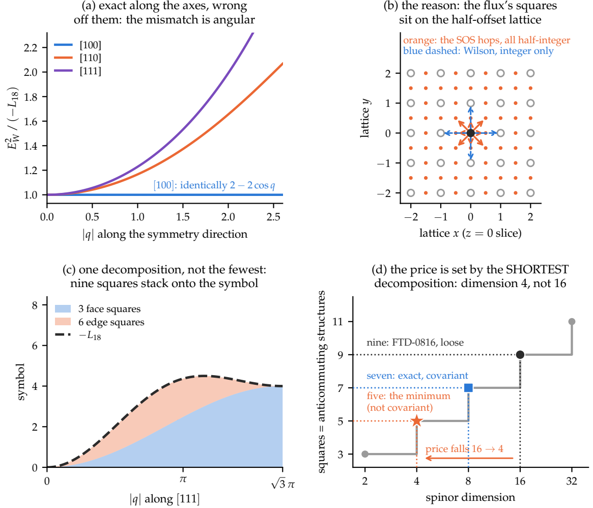
Figure 11: Why two sectors miss, and what a hit costs. (a) Normalised to a common slope, the flux symbol and a Wilson operator agree identically along the cubic axes — both are 2 - 2 \cos q — and diverge only off them, reaching 1.65 along [110] and 1.99 along [111] at |q| = 2 . The mismatch is purely angular, so no rescaling is even the right shape. (b) The reason, in the z = 0 slice: the flux symbol's nine squares carry arguments q_i/2 and (q_i \pm q_j)/2 , i.e. hops of half a lattice unit (orange), while Wilson hops land on integer sites (blue dashed). The sectors were being matched on different lattices. (c) One such identity: three face squares and six edge squares stack exactly onto -L_{18} , with residual 1.8 \times 10^{-15} over 4000 random momenta. (d) The price, which is set by the shortest decomposition rather than by any one of them. n squares require n mutually anticommuting structures and dimension 2^k carries 2k + 1 , so nine would cost spinor dimension 16; but nine is not the fewest. An exact cubic-covariant seven -square identity holds, -L_{18} = 4 \sum_i \sin^2 x_i \cos^2 x_j \cos^2 x_k + \frac{16}{3} \sum_i \sin^2 x_j \sin^2 x_k \cos^2 x_i + 4 \sin^2 x_1 \sin^2 x_2 \sin^2 x_3 with x = q/2 , costing dimension 8; and a search over the nearest-neighbour class finds a five at dimension 4 — ordinary Dirac — which is genuinely non-covariant. The fourfold taste multiplication was an artefact of a non-minimal decomposition, not a feature of the symbol.
