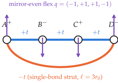
(a) the minimum viable carrier: \omega = (1, 1, 1, -1)
