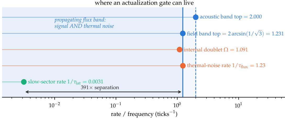
Figure 7: Why the negative was structural rather than accidental. The propagating band carries both the signal modes and the thermal noise, so the noise rate cannot be pushed below the band. Only a channel outside that band — here the model’s slowly accumulating gravitational-potential sector, three orders of magnitude slower — sits where an actualization gate would have to sit.
