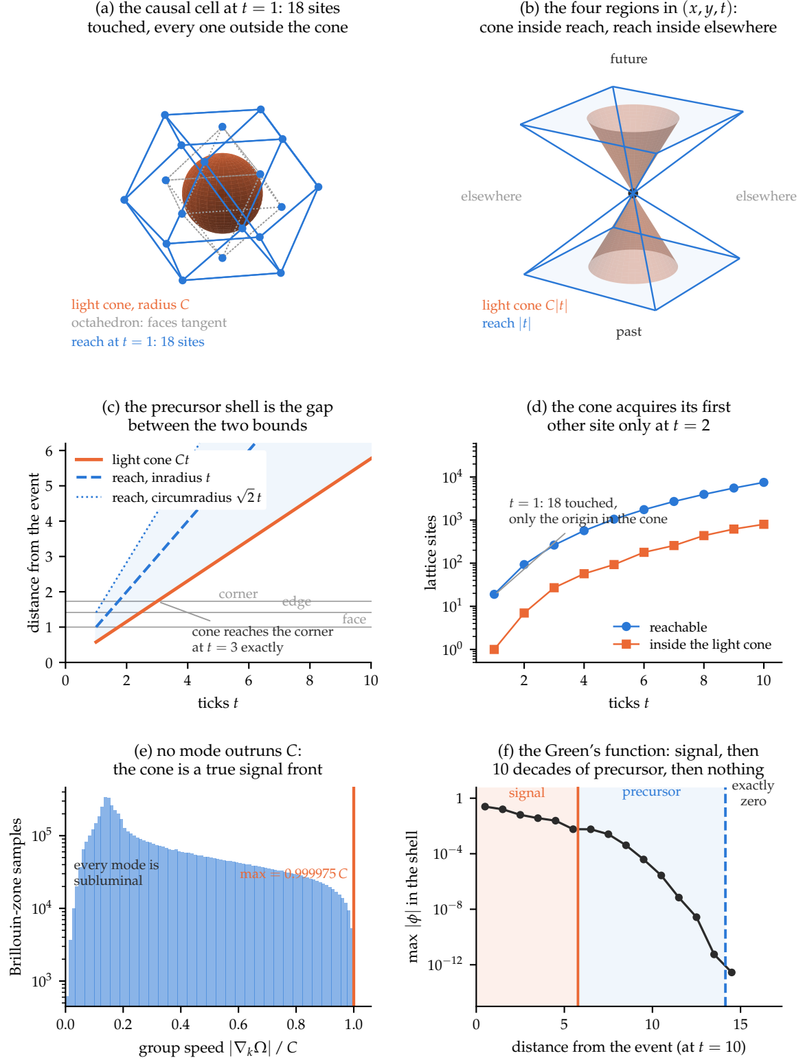
Figure 15: The complete causal partition around one event. (a) At t = 1 the light-cone sphere is inscribed in the octahedron — its inradius is C , so the eight faces are tangent — which is itself inside the reach polytope. (b) Past, future, and elsewhere in (x, y, t) , with the round cone strictly inside the square-sectioned reach. (c) The precursor shell is the gap between the two bounds; the cone closes over the body diagonal at t = 3 exactly. (d) At t = 1 eighteen sites have been touched and only the origin lies in the cone. (e) Every finite-wavelength mode is strictly subluminal, so the cone is a true signal front. (f) Across the shell the Green's function falls ten decades and then terminates in an exact zero.
