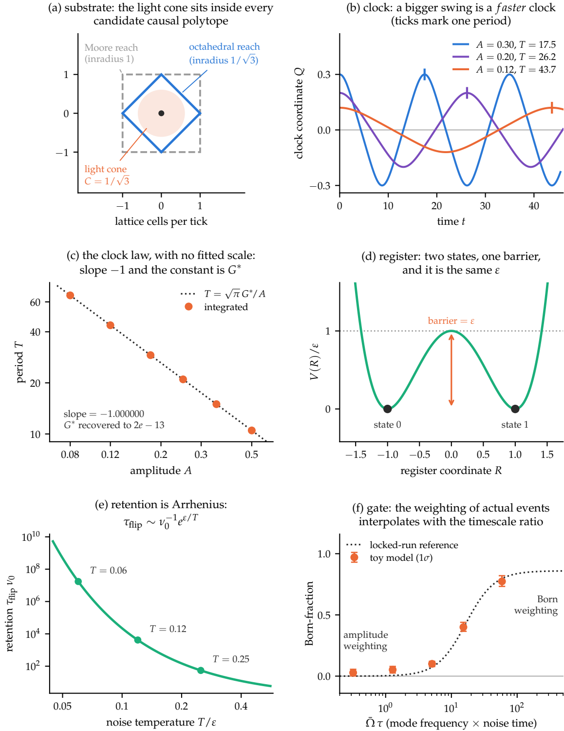
Figure 14: The minimal temporal interior, computed end to end. (a) The light cone at C = 1/\sqrt{3} lies inside the octahedral reach and hence inside every candidate causal polytope. (b) Unscaled clock trajectories: amplitudes differing by 2.5\times give periods differing by the reciprocal factor — a bigger swing is a faster clock. (c) The same integration on log axes recovers slope exactly -1 and the constant G^* to 1.6 \times 10^{-13} , with nothing fitted. (d) The register’s barrier equals its well depth exactly. (e) Retention is Arrhenius in that same \varepsilon . (f) The weighting of actual events interpolates from amplitude to occupation as \bar{\Omega}\tau grows, with 1\sigma bootstrap intervals shown rather than suppressed; the dotted curve is the locked-run descriptive reference of Figure 6.
