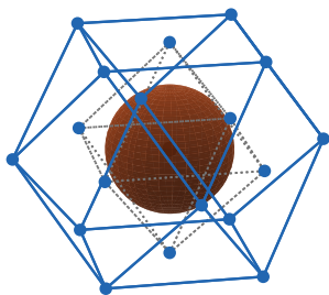
light cone, radius C octahedron: faces tangent reach at t = 1 : 18 sites
