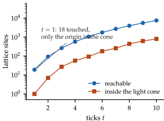
(d) the cone acquires its first other site only at t = 2
