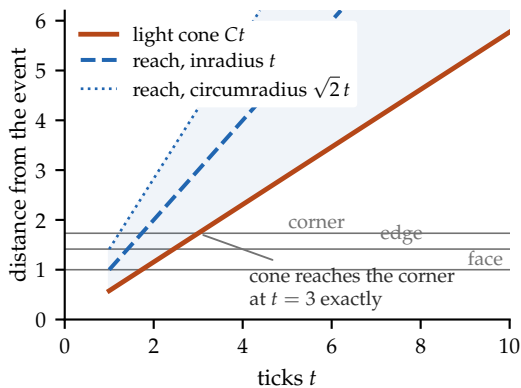
(c) the precursor shell is the gap between the two bounds
