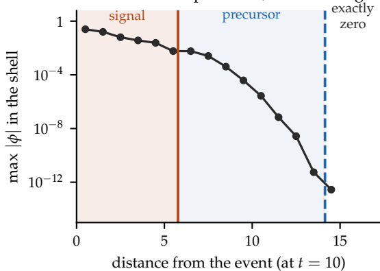
(f) the Green's function: signal, then 10 decades of precursor, then nothing
