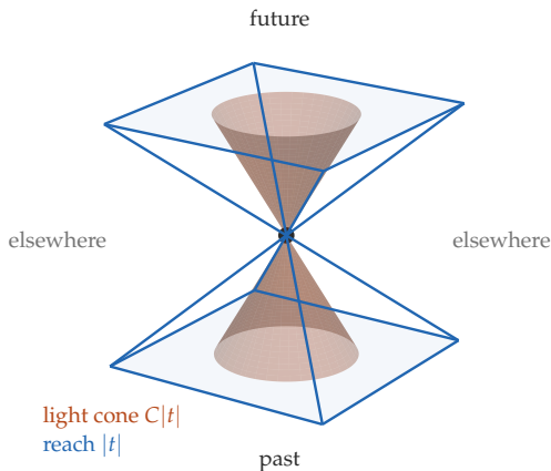
(b) the four regions in (x, y, t) : cone inside reach, reach inside elsewhere
