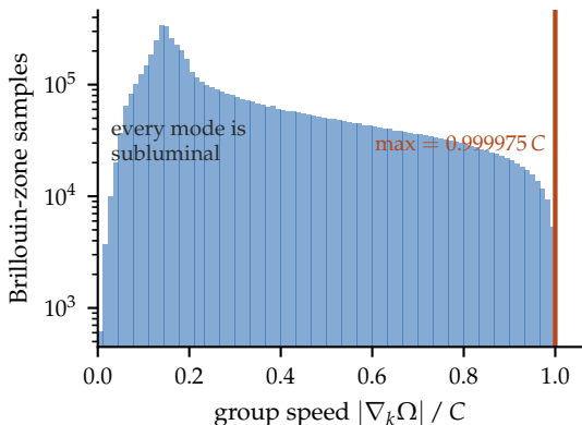
(e) no mode outruns C : the cone is a true signal front
