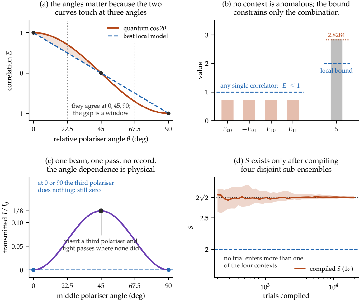
Figure 14: The angles, and the boundary. (a) For polarisation-entangled light the quantum correlation \cos 2\theta and the best local model — a straight line — touch at 0^\circ , 45^\circ and 90^\circ , so the violation is an angle window rather than a uniform excess; the widest single gap is 0.211 at 19.85^\circ . (b) At the CHSH settings each of the four contexts contributes exactly 1/\sqrt{2} , well inside the |E| \leq 1 available to any correlator: no context is individually anomalous, and the local bound constrains only the total. (c) Two crossed polarisers transmit nothing; inserting a third at 45^\circ transmits I_0/8 . One beam, one pass, no ensemble comparison and no record — the angle dependence is physical, not a feature of the bookkeeping. (d) S by contrast is a compiled statistic: the four sub-ensembles are verified disjoint and exhaustive, no trial enters more than one, and the number exists only after all four are combined.
