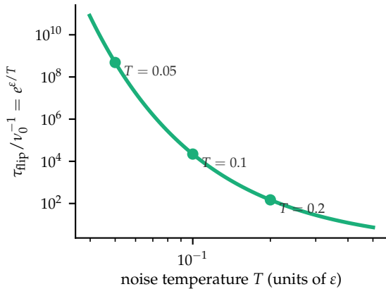
(b) retention is Arrhenius in the same \varepsilon
