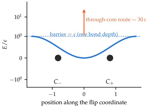
(a) the geometric bit: two states, barrier \varepsilon
