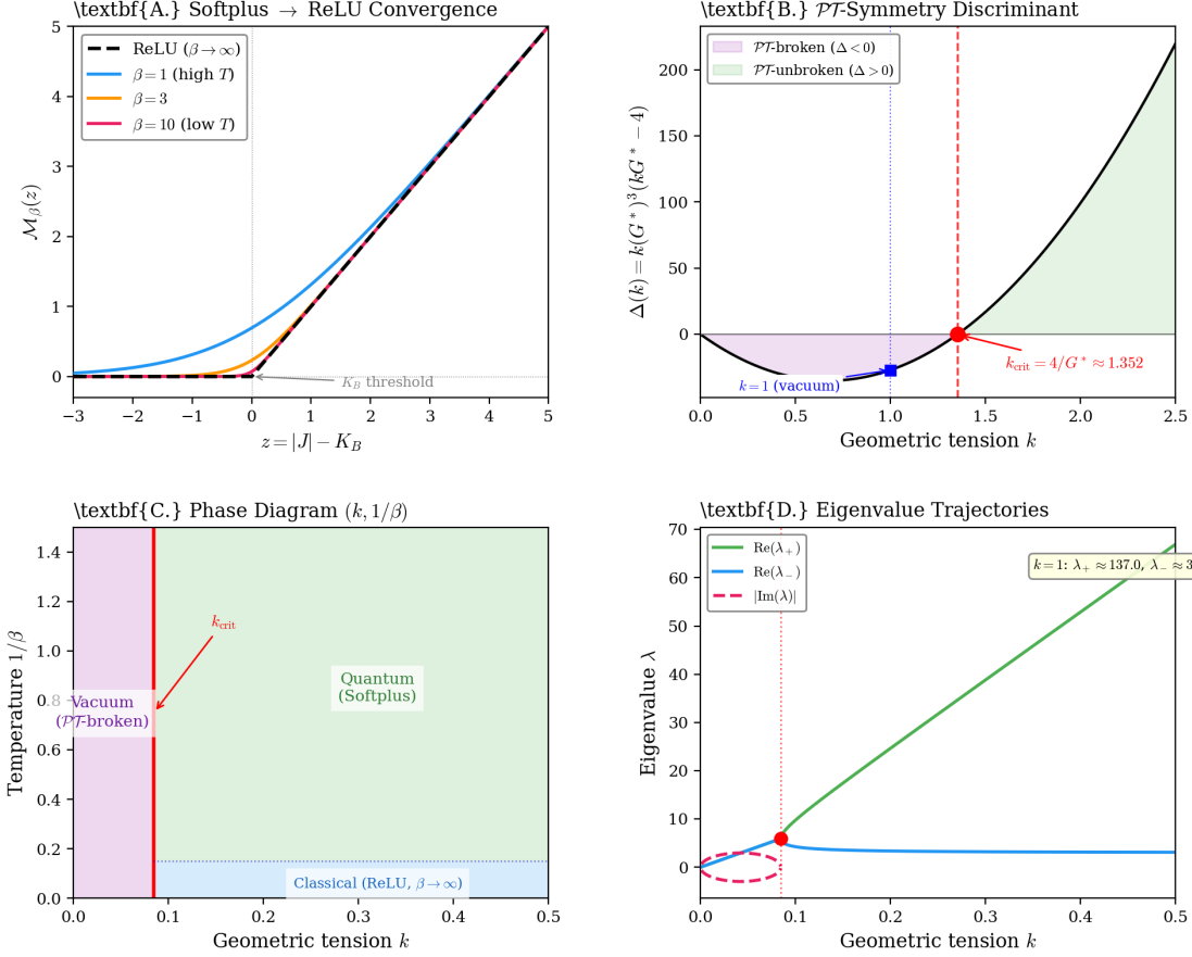
Figure 1: The Softplus-ReLU phase structure. (A) The Softplus \mathcal{M}_\beta(z) at three temperatures, converging mathematically to ReLU as \beta \rightarrow \infty . (B) The discriminant \Delta(k) in the n = 1 sector, locating the \mathcal{PT} -boundary exactly at k_{\text{crit}} = 4/G^* \approx 1.352 . (C) The (k, 1/\beta) phase diagram mapped in the n = 16 sector ( k_{\text{crit}} = 1/(4G^*) \approx 0.085 ), denoting the physical vacuum resting at k = 1 . (D) Eigenvalue trajectories ( n = 16 ) tracking k variations; notably at k = 1 , eigenvalues split strictly to \lambda_+ \approx 137.04 and \lambda_- \approx 3.02 .
