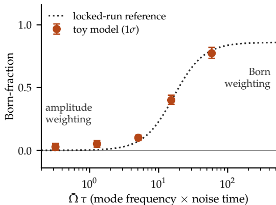
(f) gate: the weighting of actual events interpolates with the timescale ratio
