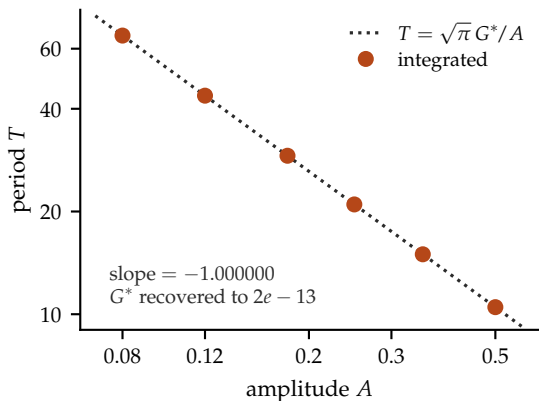
(c) the clock law, with no fitted scale: slope -1 and the constant is G^*
