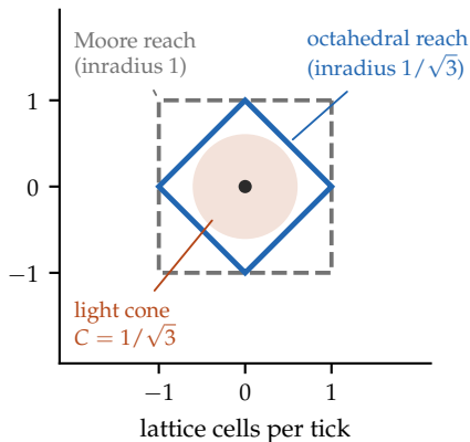
(a) substrate: the light cone sits inside every candidate causal polytope
