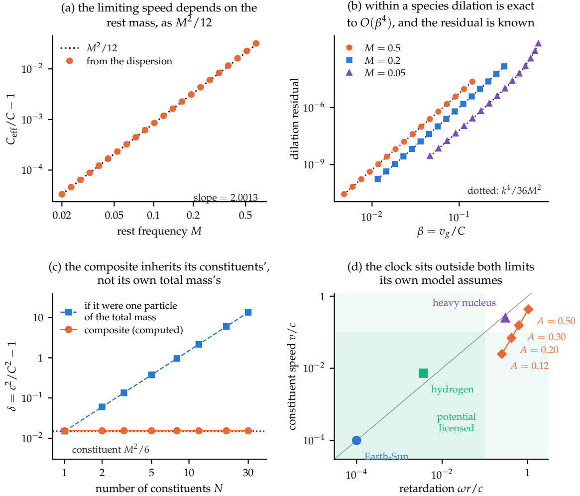
Figure 13: The cone arc of Sections 9.7–9.10, computed. (a) The limiting speed extracted from the exact dispersion tracks M^2/12 ; the fitted log–log slope is 2.0013. (b) Using each species’ own C_{\text{eff}} , the dilation relation fails only at O(\beta^4) , and the residual follows the analytic k^4/36M^2 (dotted) to within 1.1% across three masses. (c) The composite result: a bound object’s excess is its constituents’, constant to seven digits as the constituent number runs 1 \rightarrow 30 , while the reading that treats it as one particle of the total mass grows as N^2 . (d) The two limits hidden in a distance potential, with real systems placed. Orbits lie on the diagonal because \omega r = v for them; the mechanical clock does not, and sits outside the licensed corner on both axes — more relativistic internally than a heavy nucleus.
