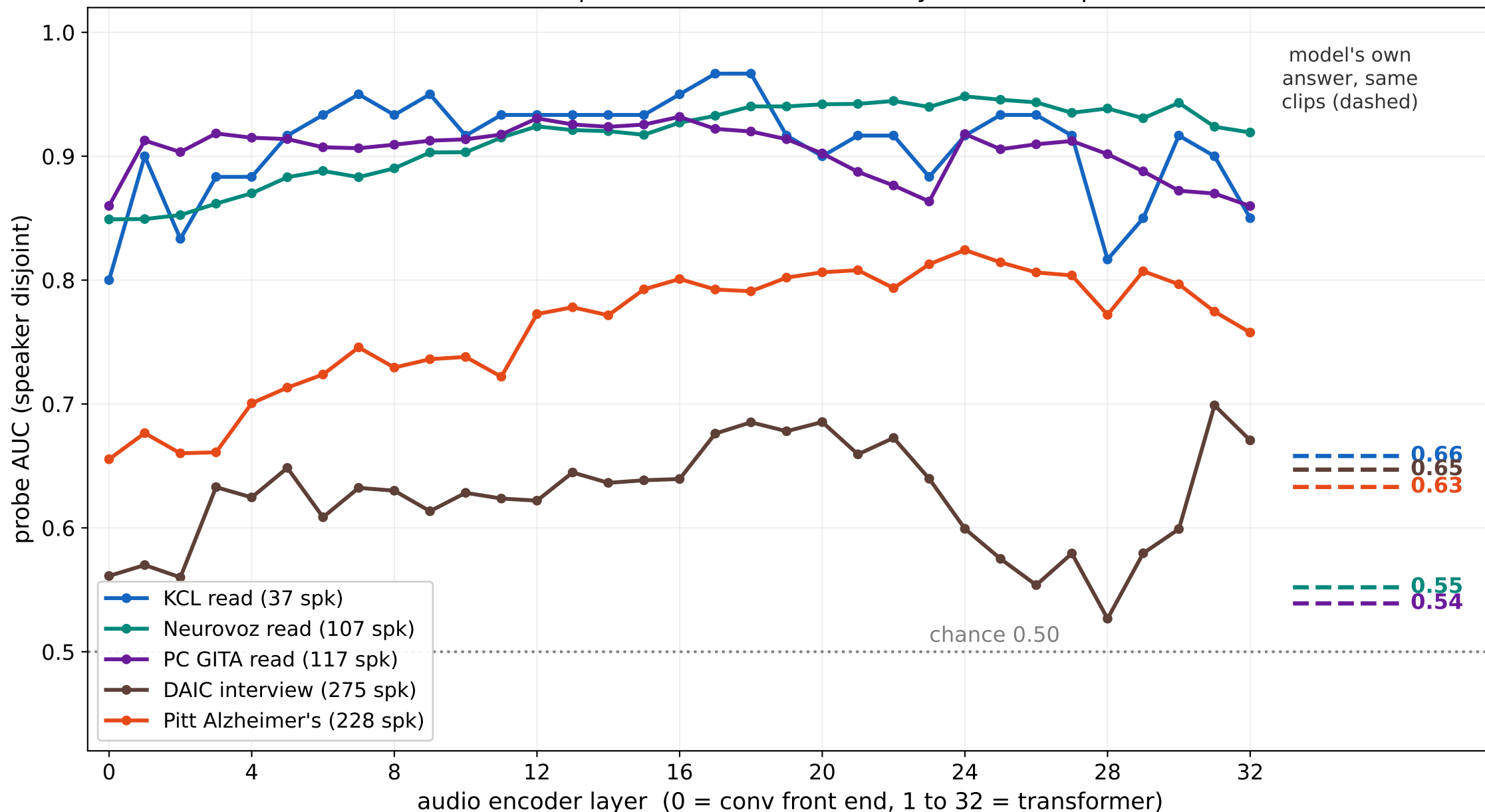
qwen2 audio encoder, one linear probe per layer, all 33 layers within dataset, whole speakers held out, audio only, no transcript, 30 s windows
