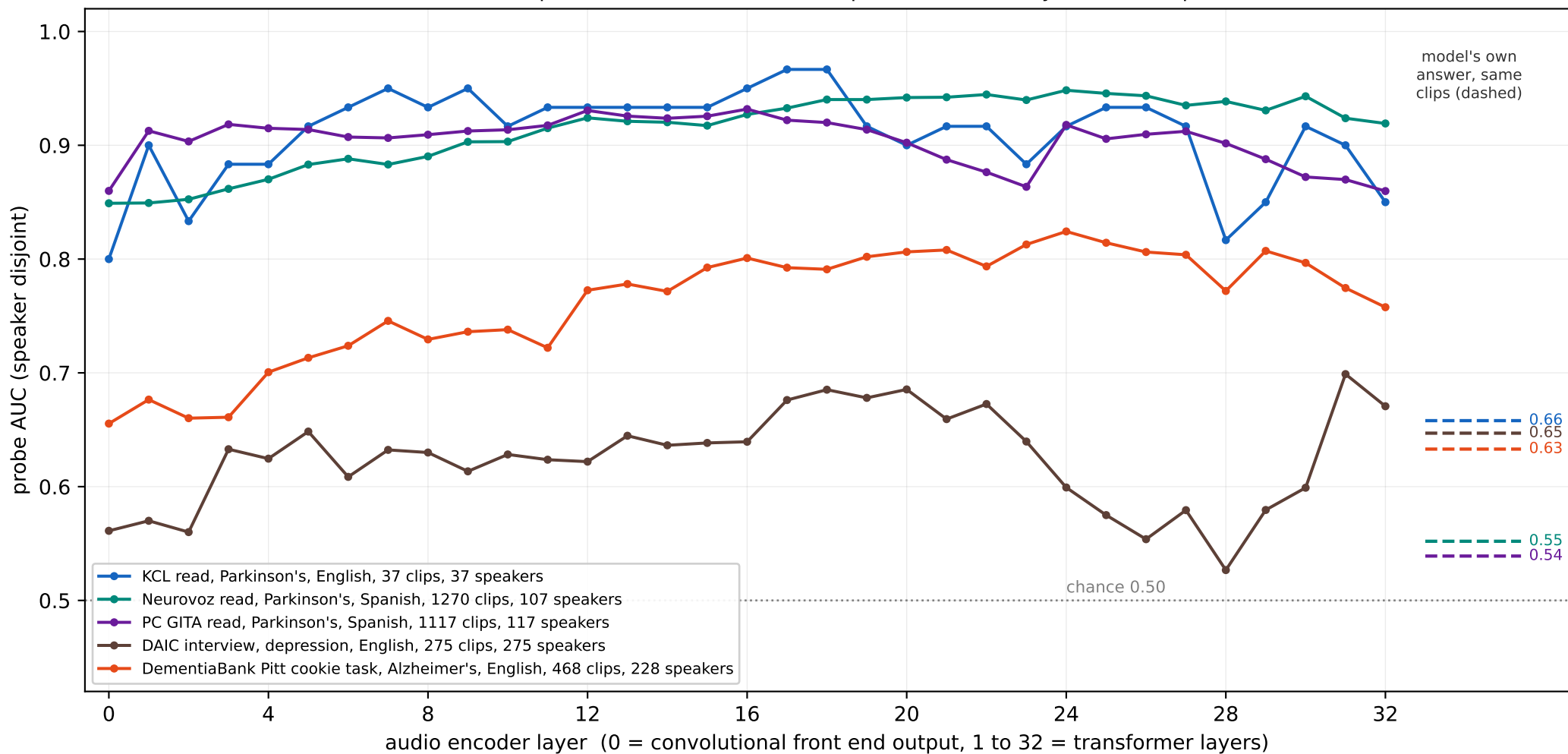
qwen2 audio encoder, one linear probe per layer, all 33 layers within dataset, whole speakers held out (5 fold GroupKFold), audio only, no transcript, 30 s windows
