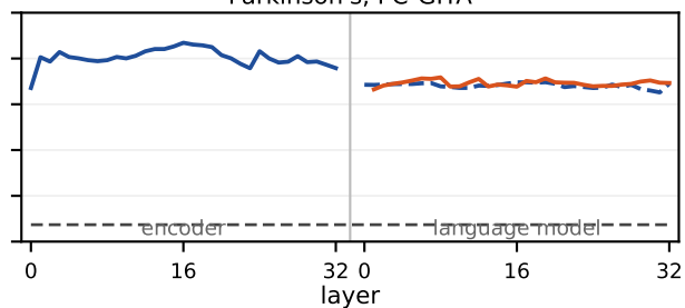
Parkinson's, PC-GITA
