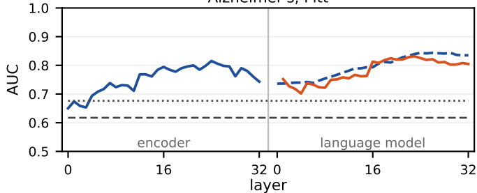
Alzheimer's, Pitt
