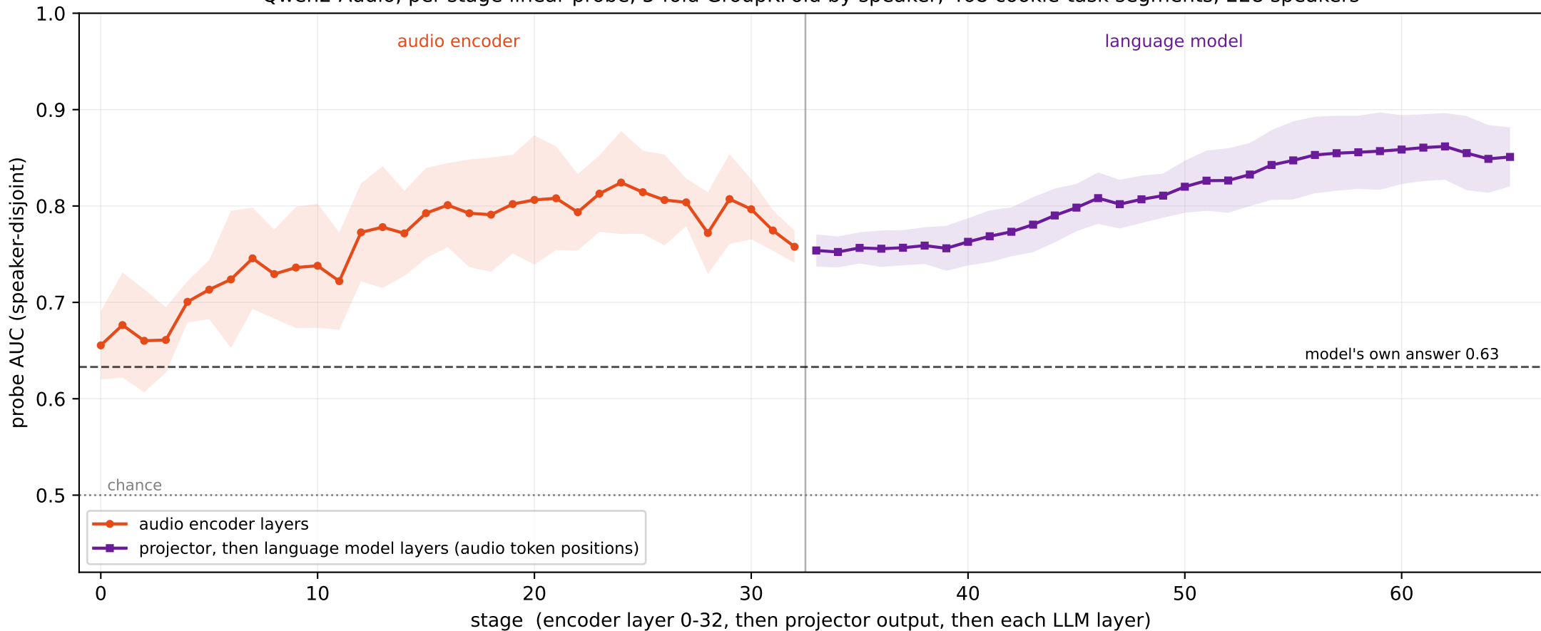
Alzheimer's (DementiaBank Pitt): disease information from the audio encoder through the language model Qwen2-Audio, per-stage linear probe, 5-fold GroupKFold by speaker, 468 cookie-task segments, 228 speakers
