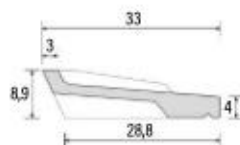
Appui carré R 330
