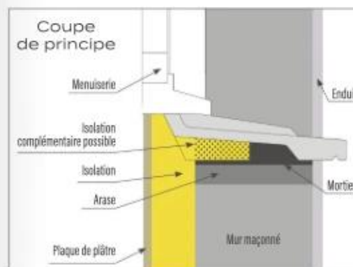
Appui carré R 360
