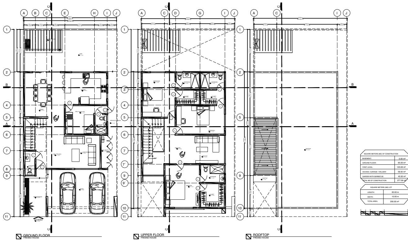
ARCHITECTURAL PLAN Ground floor, first floor and ROOFTOP floor
