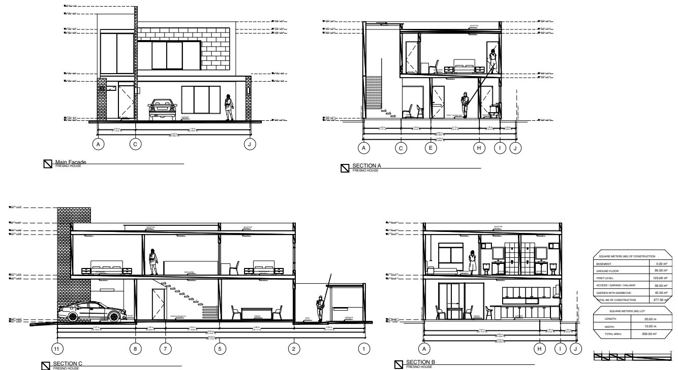
ARCHITECTURAL PLAN Architectural facades and sections
