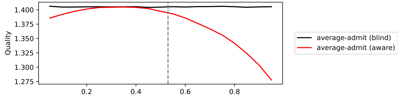
Quality of Class in Polyculture ( m = 4 )
