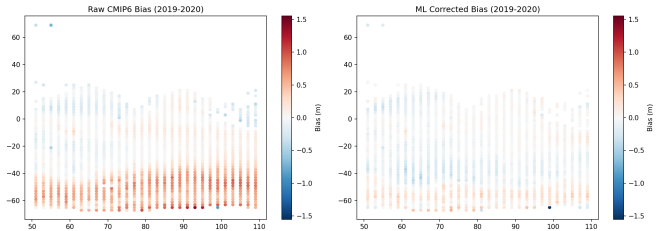
Fig. 13: SWH spatial bias maps (2019–2020). Left: raw CMIP6 bias showing widespread overestimation. Right: ML-corrected bias reduced to near zero.
