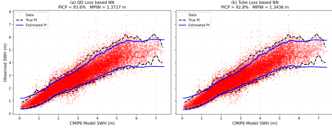
Fig. 16: SWH prediction intervals: (a) QD Loss and (b) Tube Loss. Red dots: data. Black dashed: empirical true PI. Blue solid: estimated PI. The SWH dataset shows smoother PI estimation due to the larger sample size.
