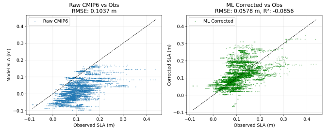
Fig. 2: Scatter plots of observed vs. predicted SLA for the test period. Left: Raw CMIP6 model. Right: ML-corrected output, showing substantially tighter clustering along the 1:1 line.
