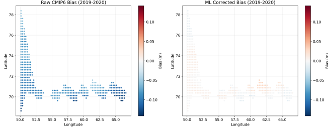
Fig. 4: Spatial bias maps for the test period (2019–2020). Left: raw CMIP6 model bias. Right: ML-corrected bias. The correction substantially reduces spatially structured errors.
