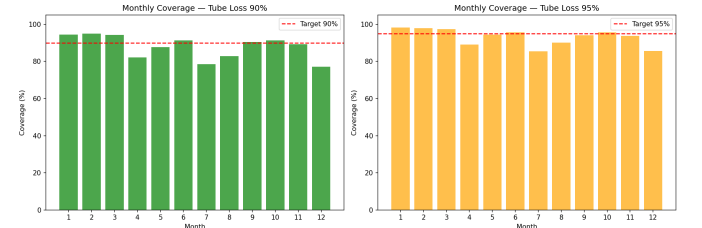
Fig. 15: SWH monthly PICP for Tube Loss 90% and 95% PIs. Coverage is relatively uniform across months, with slightly lower coverage during high-variability winter months.
