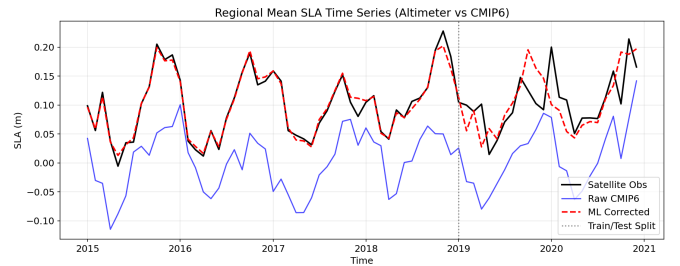
Fig. 3: Regional mean SLA time series. Black: satellite observations. Blue: raw CMIP6 model. Red dashed: ML-corrected. The vertical grey line marks the train/test split.
