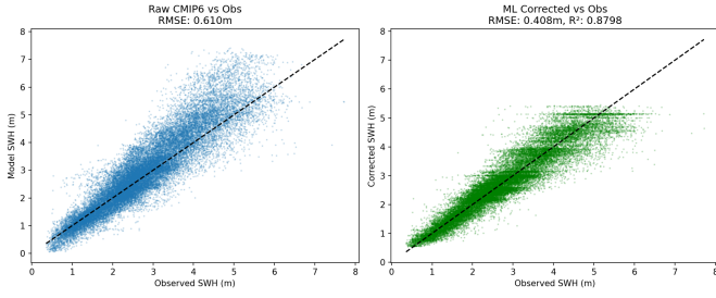
Fig. 11: SWH scatter plots. Left: Raw CMIP6 vs observations (RMSE 0.610m). Right: ML-corrected vs observations (RMSE 0.408m, R^2=0.88 ), showing substantially tighter clustering.
