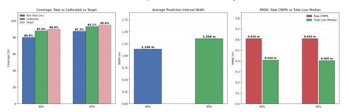
Fig. 18: SWH three-panel summary: (a) coverage comparison, (b) average PI width, (c) RMSE comparison showing 33% improvement over raw CMIP6.
