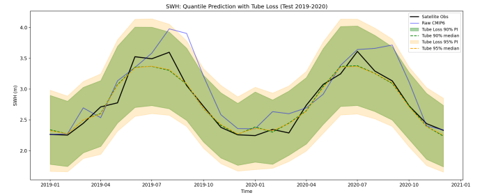
Fig. 14: SWH time series with Tube Loss prediction intervals. Green/orange bands: 90%/95% calibrated PIs. The intervals capture the seasonal amplitude variations.
