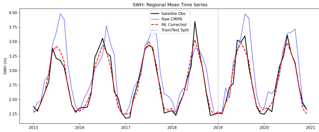
Fig. 12: SWH regional mean time series. The ML-corrected curve (red dashed) closely follows satellite observations (black), correcting the systematic overestimation of the raw CMIP6 model (blue).
