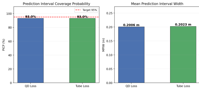
Fig. 9: Bar chart comparison of PICP (left) and MPIW (right) for QD Loss and Tube Loss after conformal calibration. Both methods achieve 93.0% coverage.
