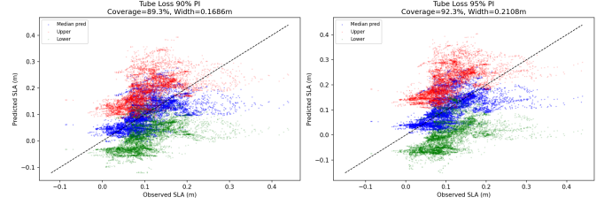
Fig. 10: Observed SLA vs. Tube Loss predictions for 90% and 95% PIs. Blue: median prediction. Red/green: upper/lower bounds. Points near the 1:1 line indicate good calibration.
