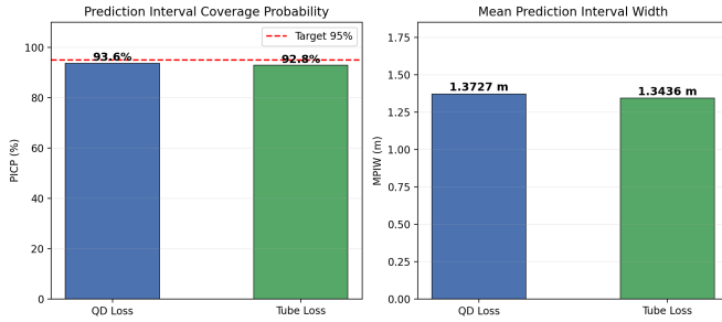
Fig. 17: SWH PICP (left) and MPIW (right) comparison. Both methods exceed 92% calibrated coverage.
