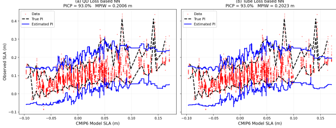
Fig. 8: Prediction intervals estimated by (a) QD Loss and (b) Tube Loss neural networks. Red dots: test data. Black dashed: empirical (true) PI. Blue solid: estimated PI. Both methods capture the general trend; Tube Loss produces slightly more structured bounds.
