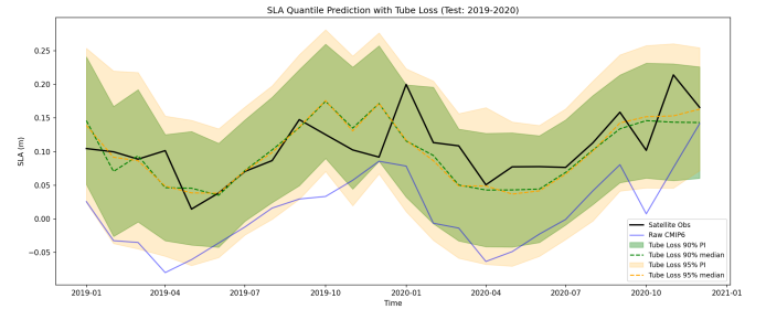
Fig. 5: SLA time series with Tube Loss prediction intervals. Green and orange bands represent 90% and 95% calibrated PIs. Dashed lines show the median prediction.
