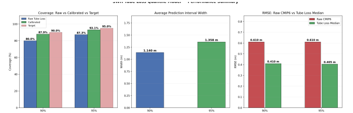
Fig. 17: SWH three-panel summary: (a) coverage comparison, (b) average PI width, (c) RMSE comparison showing 33% improvement over raw CMIP6.
