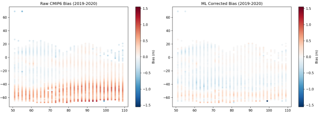
Fig. 12: SWH spatial bias maps (2019–2020). Left: raw CMIP6 bias showing widespread overestimation. Right: ML-corrected bias reduced to near zero.
