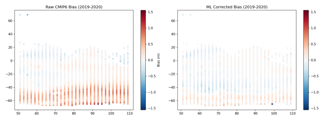
Fig. 13: SWH spatial bias maps (2019–2020). Left: raw CMIP6 bias showing widespread overestimation. Right: ML-corrected bias reduced to near zero.
