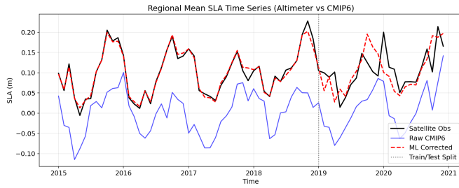
Fig. 3: Regional mean SLA time series. Black: satellite observations. Blue: raw CMIP6 model. Red dashed: ML-corrected. The vertical grey line marks the train/test split.
