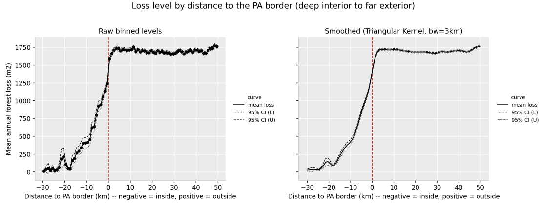
Figure 6: Loss level by distance to nearest PA boundary (deep interior to far exterior)
