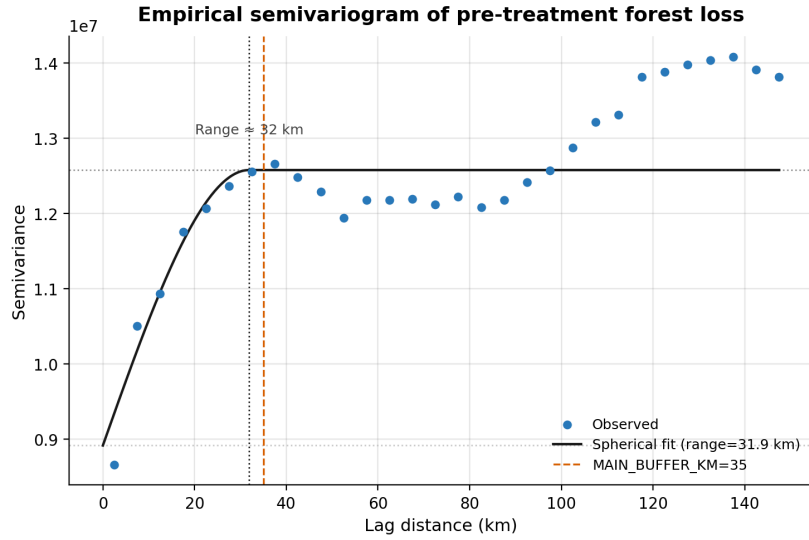
Figure 7: Empirical semivariogram of pre-treatment forest-loss
