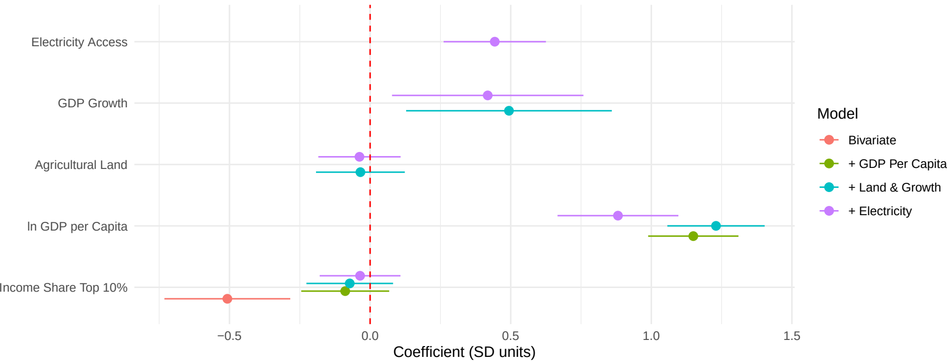
Coefficient Plot – DV: In CO2 per Capita (Standardized IVs)
