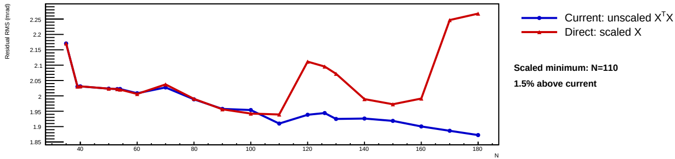
Held-out residuals, 35 \leq N \leq 180 : x'_{tar}
