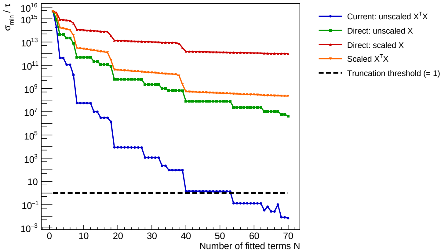
Low-N smallest singular value relative to truncation threshold
