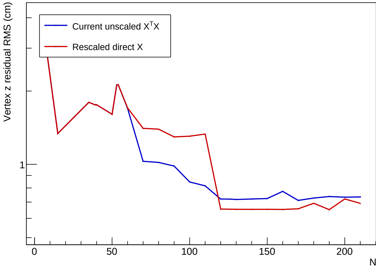
Reconstructed HMS vertex on eligible events excluded from the fit
