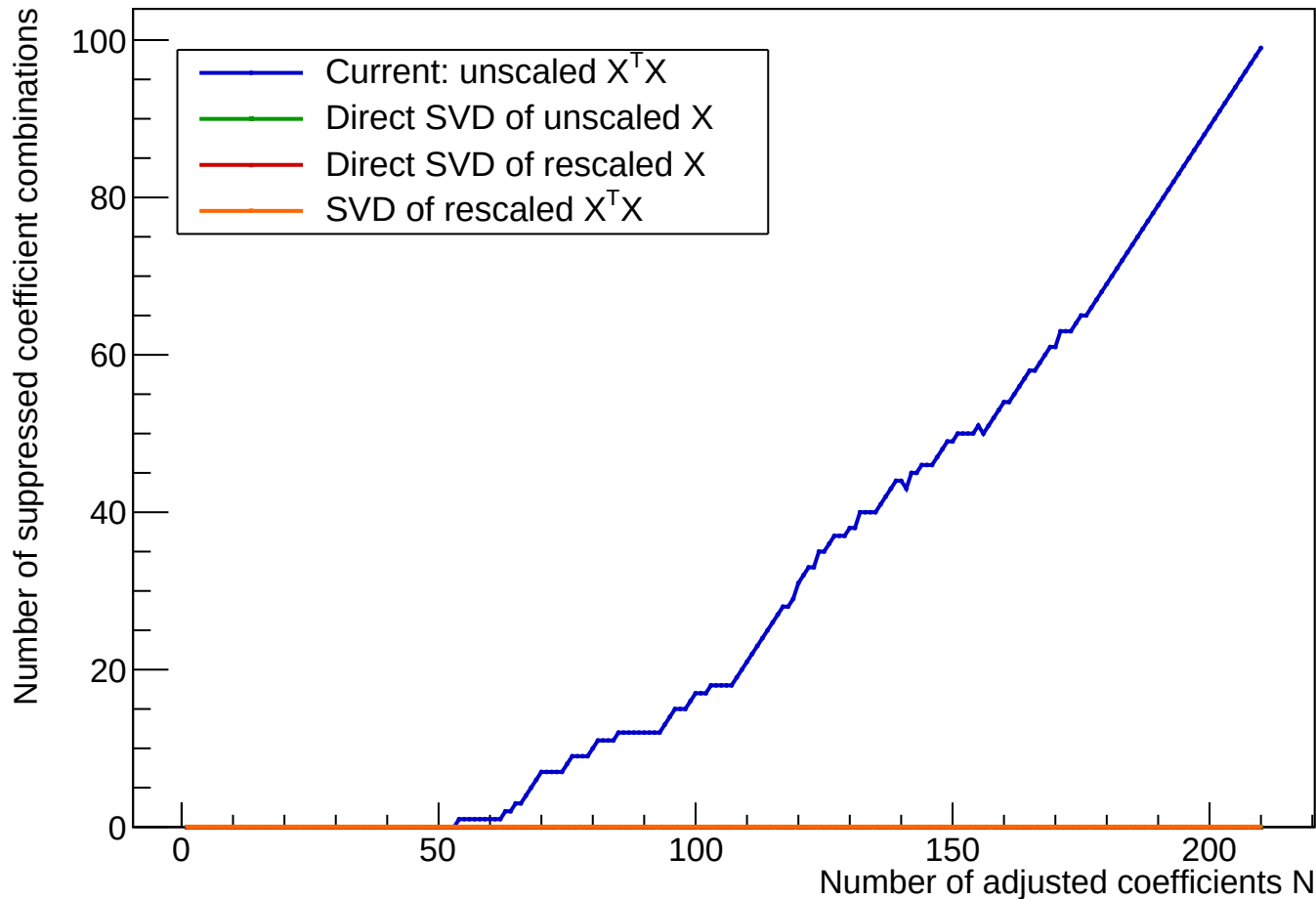
Directions suppressed by each solver's numerical cutoff
