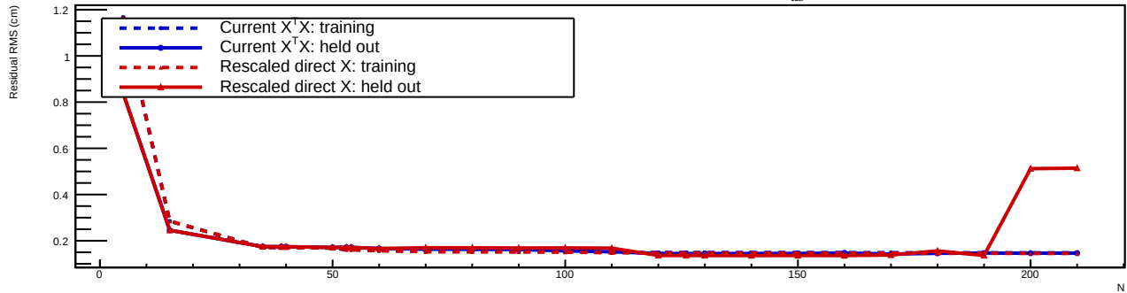
Training improvement versus held-out behavior: y'_{tar}
