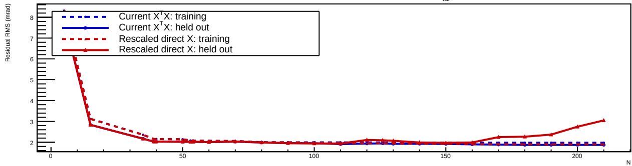
Training improvement versus held-out behavior: x'_{tar}
