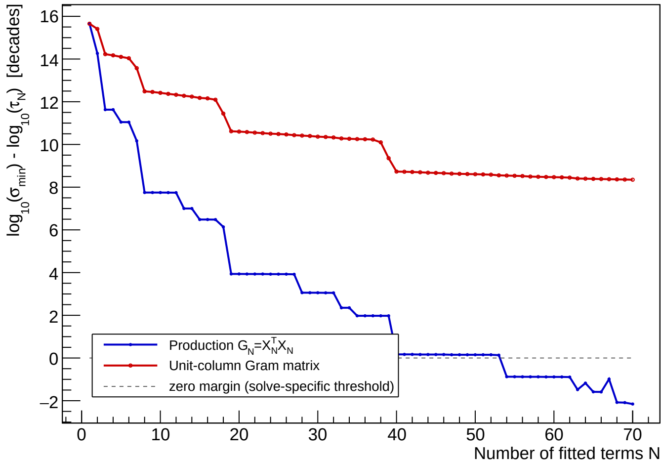
Low-N distance from each solve's own SVD threshold
