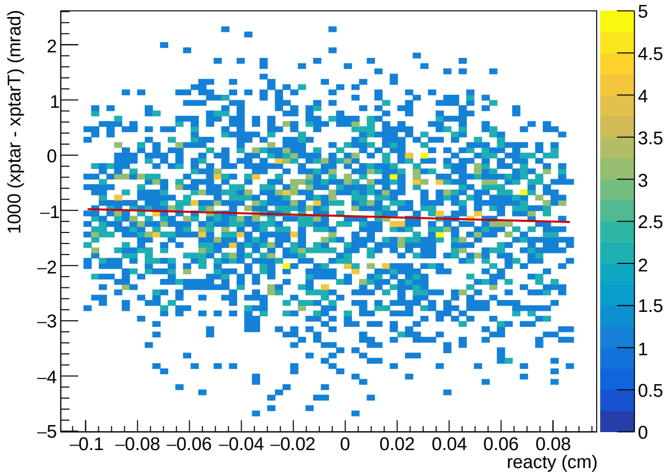
HMS rg01, 12.49 deg, foil 0 cm, hole (2, 4), inner FP core
