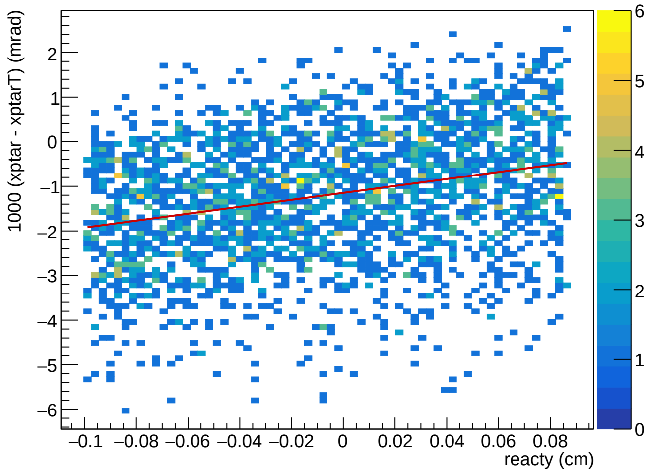
HMS rg01, 12.49 deg, foil 0 cm, hole (4, 2), core
