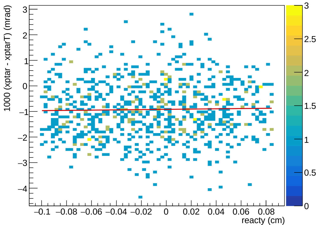
HMS rg01, 12.49 deg, foil 0 cm, hole (4, 4), inner FP core
