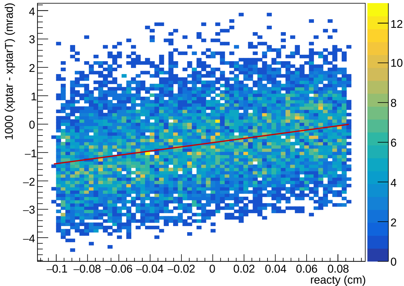
HMS rg01, 12.49 deg, foil 0 cm, hole (4, 6), core
