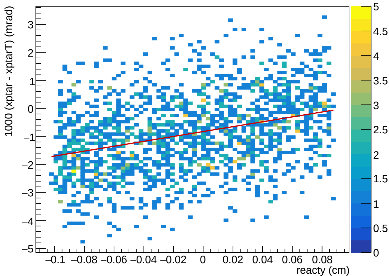
HMS rg01, 12.49 deg, foil 0 cm, hole (4, 4), core
