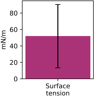
5. Surface tension
