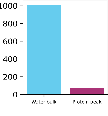
6. Density
