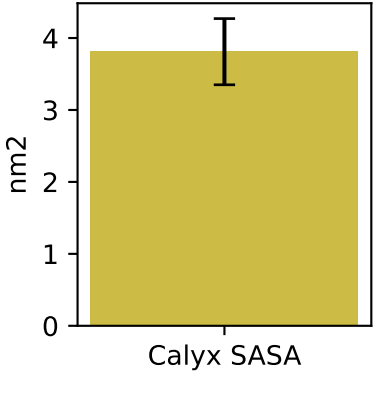
8. Calyx SASA
