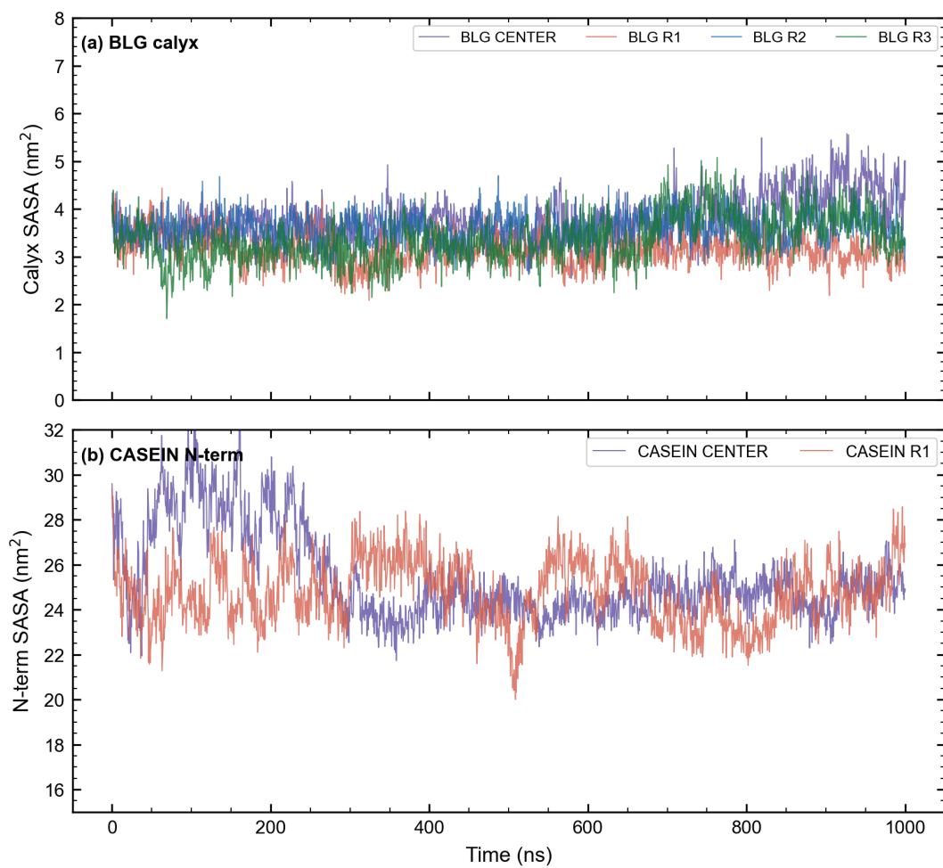
Figure 7: SASA vs. time. BLG's calyx (panel a) fluctuates in a narrow band ( \sim 2\text{--}5.5 \text{ nm}^2 ) throughout, all 4 replicas overlapping closely. CASEIN's N-terminus (panel b) fluctuates far more broadly (roughly 20\text{--}32 \text{ nm}^2 ) but never drops anywhere near BLG's range – the size gap holds at every single timepoint, not just on average.
