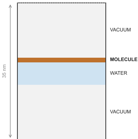
\beta -Lactoglobulin slab
