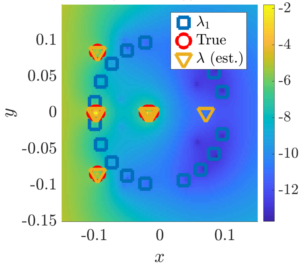
\log(\text{abs. err.})/\text{max.}
