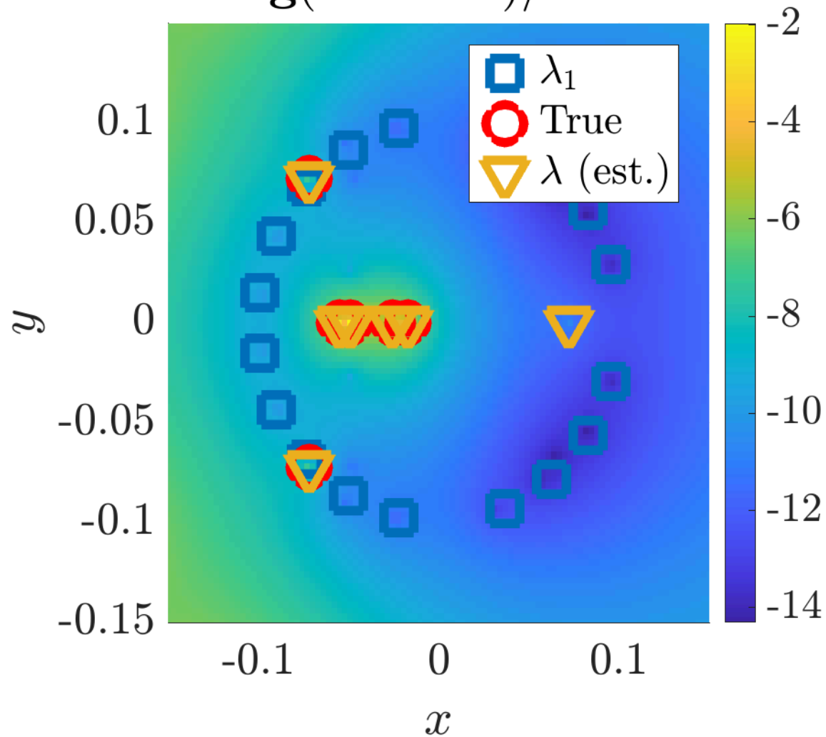
\log(\text{abs. err.})/\text{max.}
