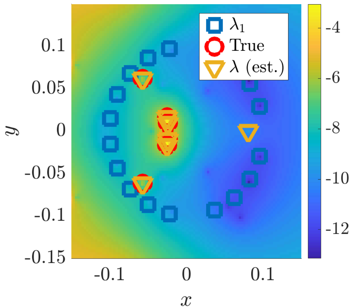
\log(\text{abs. err.})/\text{max.}
