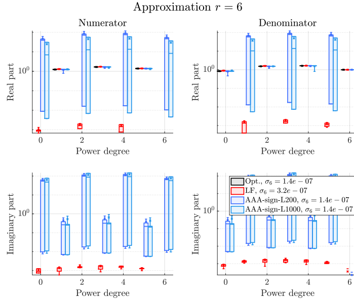
Figure 10: Case 1a, r = 6 , Z4. Numerator and denominator dispersion over the different platforms.
