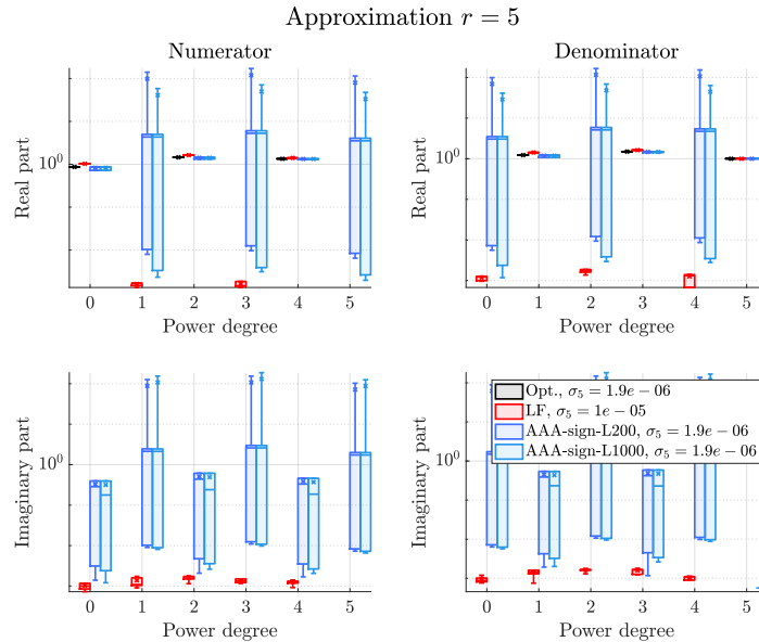
Figure 7: Case 1a, r = 5 , Z4. Numerator and denominator dispersion over the different platforms.
