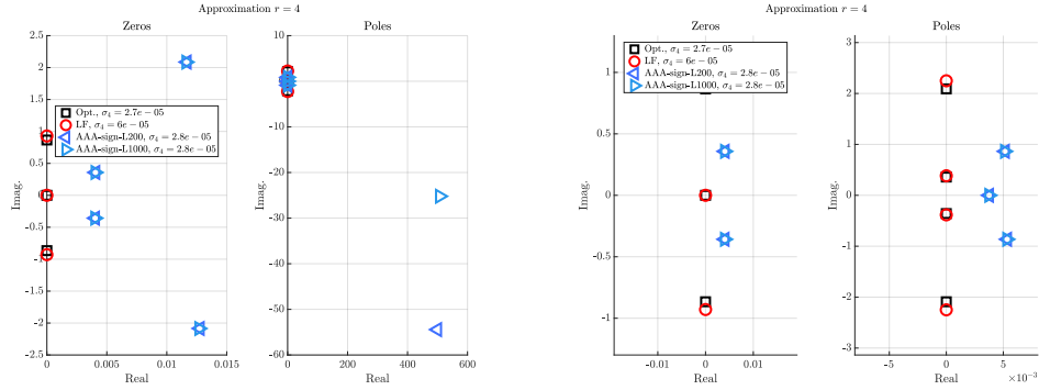
Figure 5: Case 1a (cpv MACA64 MR2023b), r = 4 , Z4. Left frame: zeros (left) and poles (right). Right frame: same but discarding the largest real entry.
