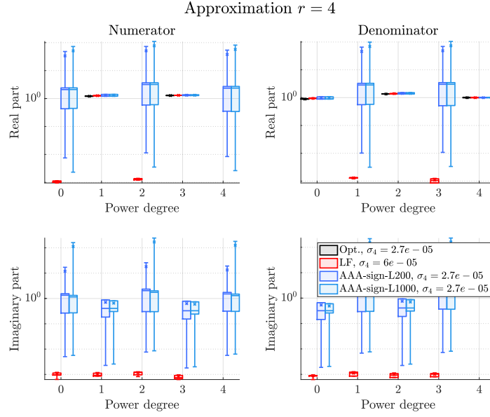
Figure 4: Case 1a, r = 4 , Z4. Numerator and denominator dispersion over the different platforms.
