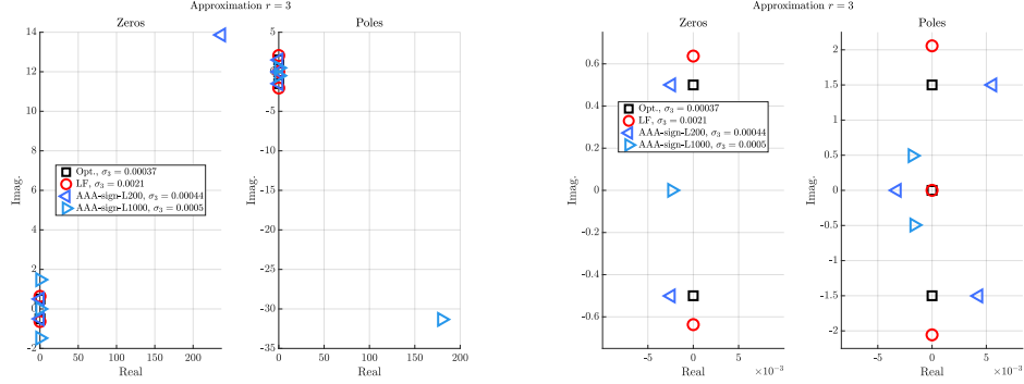
Figure 2: Case 1a (cpv MACA64 MR2023b), r = 3 , Z4. Left frame: zeros (left) and poles (right). Right frame: same but discarding the largest real entry.
