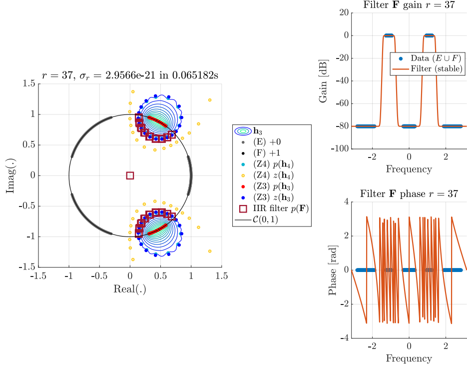
Figure 42: Bandpass filter and connection with Z4. Left: same description as fig. 1 with additionally, the mirrored poles of Z4. Right: Bode gain and phase of the obtained filter F(z) .
