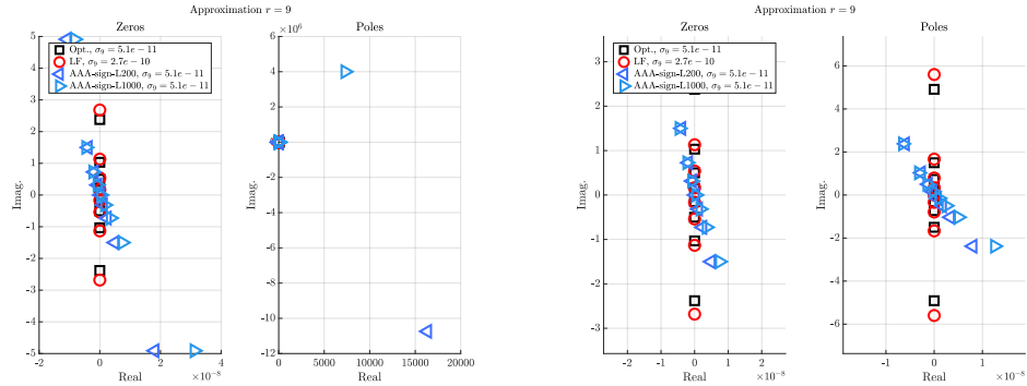
Figure 25: Case 1a (cpv MACA64 MR2023b), r = 9 , Z4. Left frame: zeros (left) and poles (right). Right frame: same but discarding the largest real entry.
