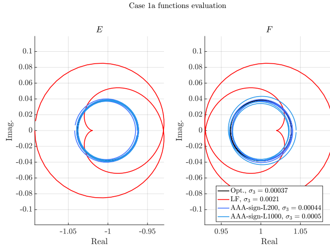
Figure 2: Case 1a (cpv MACA64 MR2023b), r = 3 , Z4. E and F evaluations.
