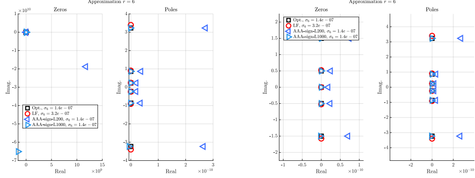
Figure 16: Case 1a (cpv MACA64 MR2023b), r = 6 , Z4. Left frame: zeros (left) and poles (right). Right frame: same but discarding the largest real entry.
