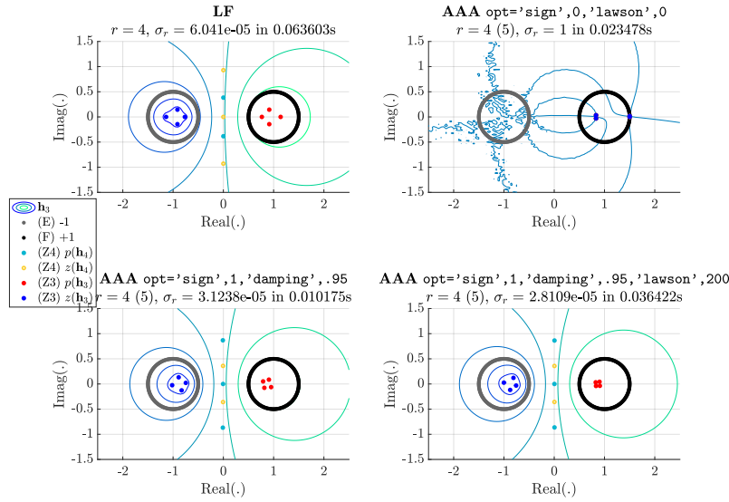
Figure 1: Case '1a', with r = 4 : different approximation methods: LF (top left), AAA (top right), AAA with damping (bottom left), and AAA-Lawson with damping and 200 iterations (bottom right). Each frame shows: the Zolotarev rational functions of degree r for Z3 ( \mathbf{h}_3 ) and Z4 ( \mathbf{h}_4 ) defined by connected sets E (on the left) and F (on the right); the Z3 function approximate contours levels \log_{10} |\mathbf{h}_3(z)| = 0, -1, -2, \dots, -30 between the two domains; yellow circles and cyan blue dots respectively mark zeros and poles of the sign function \mathbf{h}_4 ; blue and red dots respectively denote the zeros and poles of \mathbf{h}_3 . The minimum values \sigma_r and computation time are given in the title, as well as the options of each AAA method. The number of singularities targeted (and obtained).
