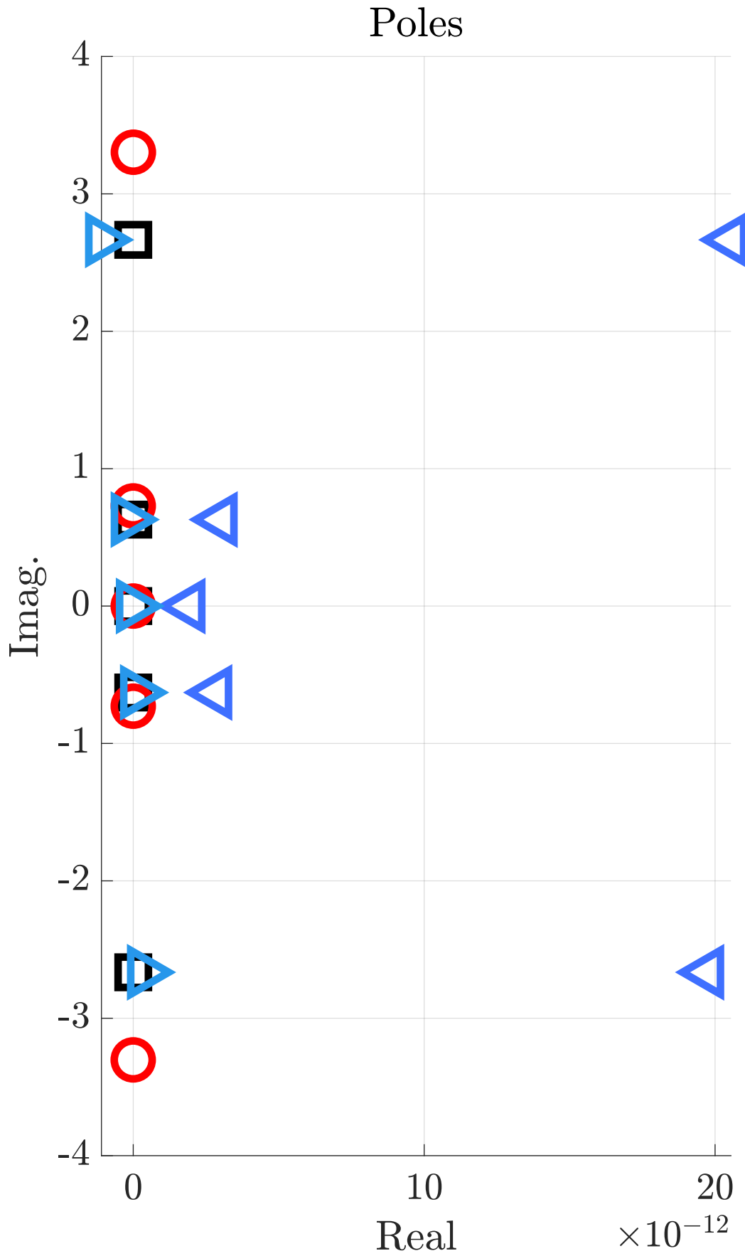
Approximation r = 5
