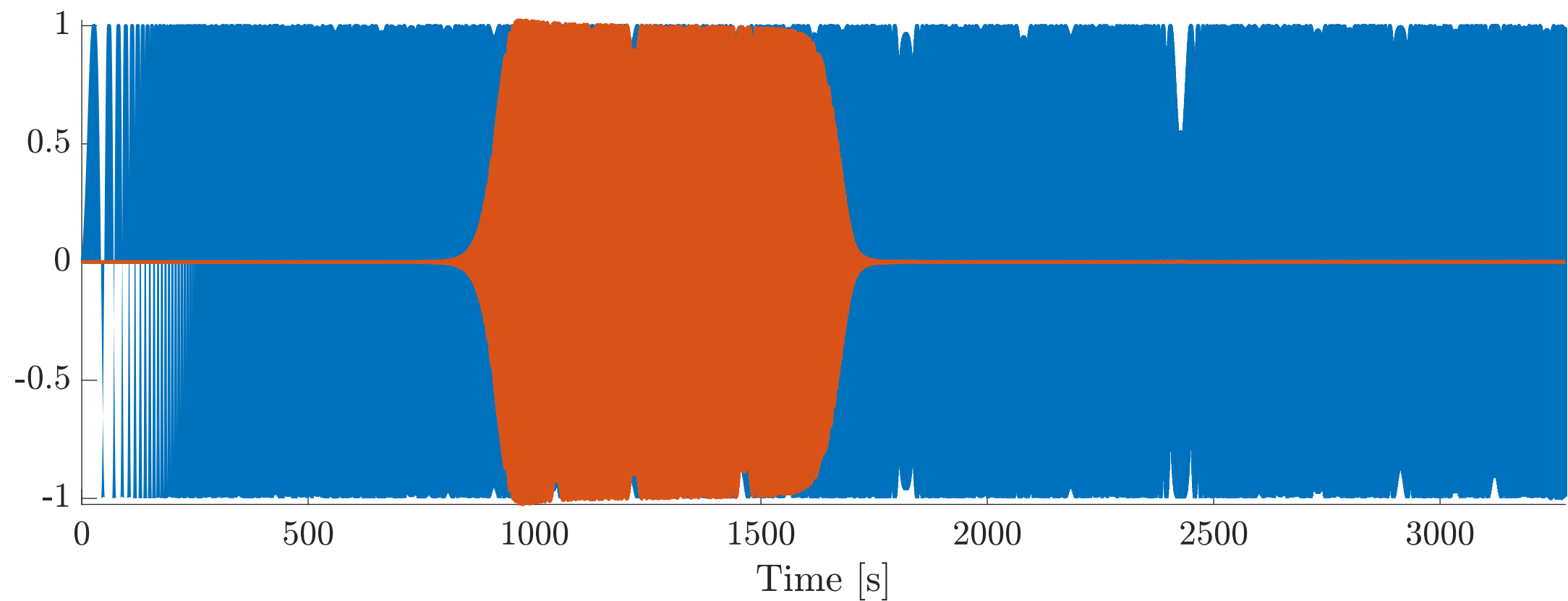
LF filter applied to chirp signal
