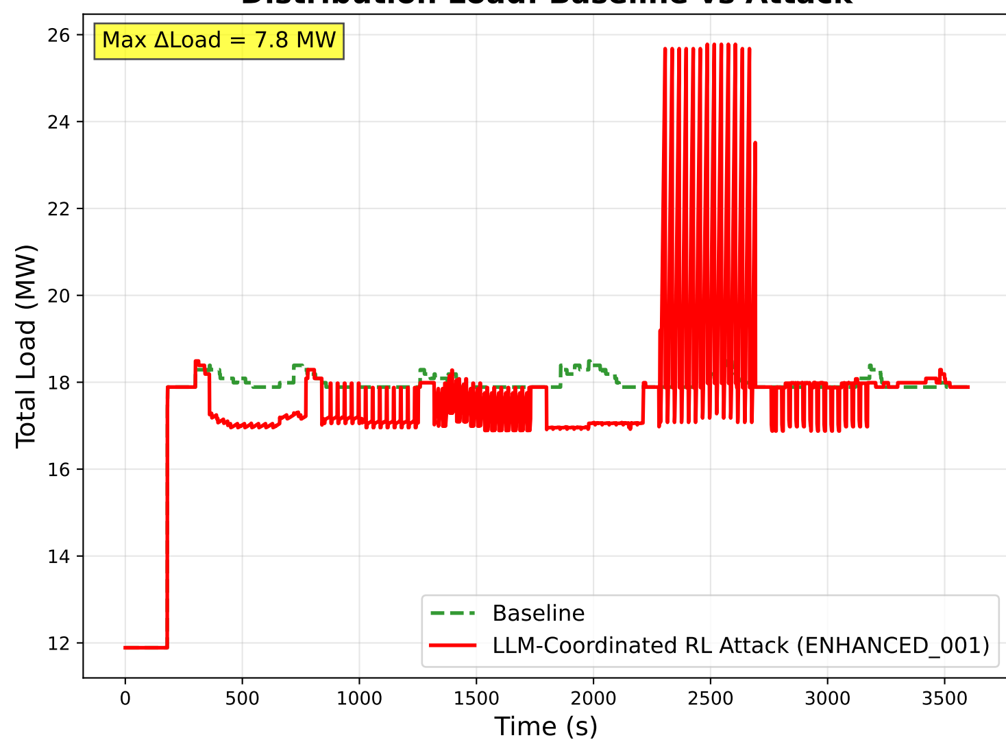
Attack Impact on Load
