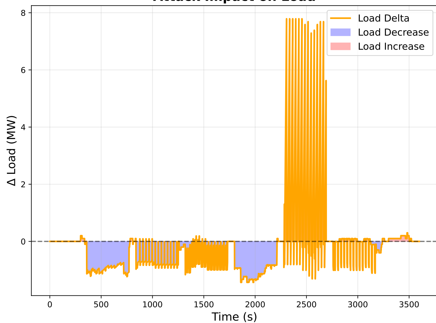
Attack Impact on Load
