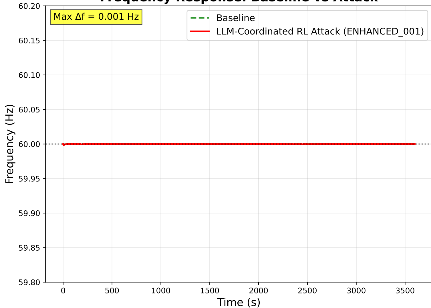
Attack Impact on Frequency
