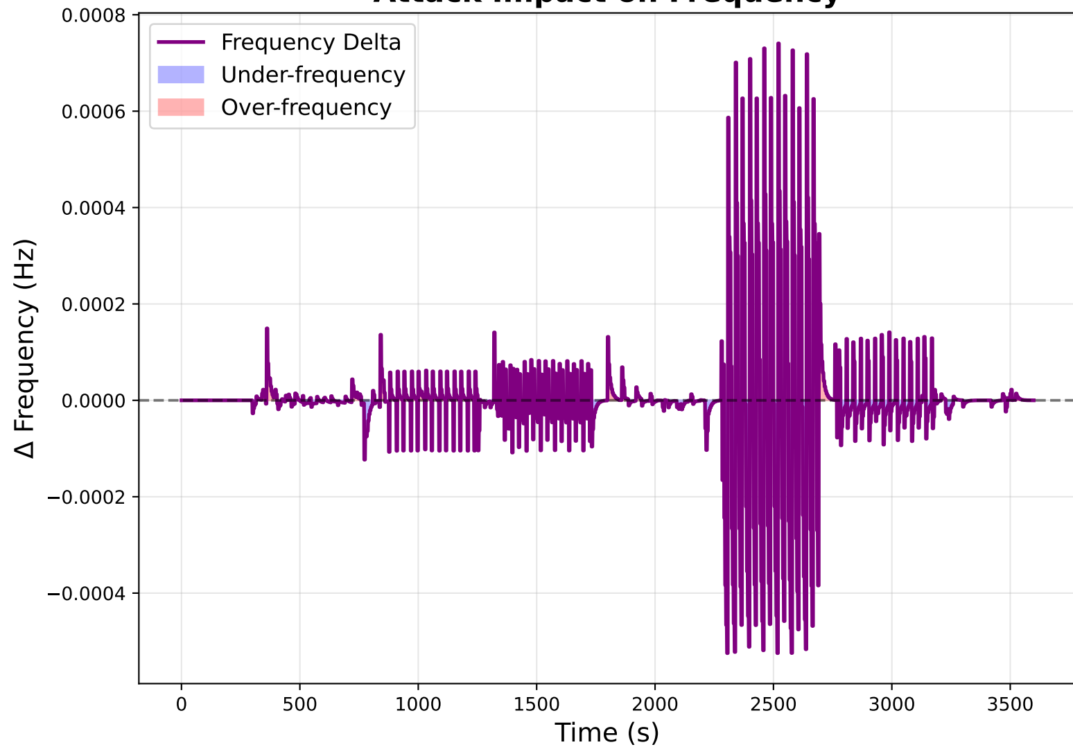
Attack Impact on Frequency
