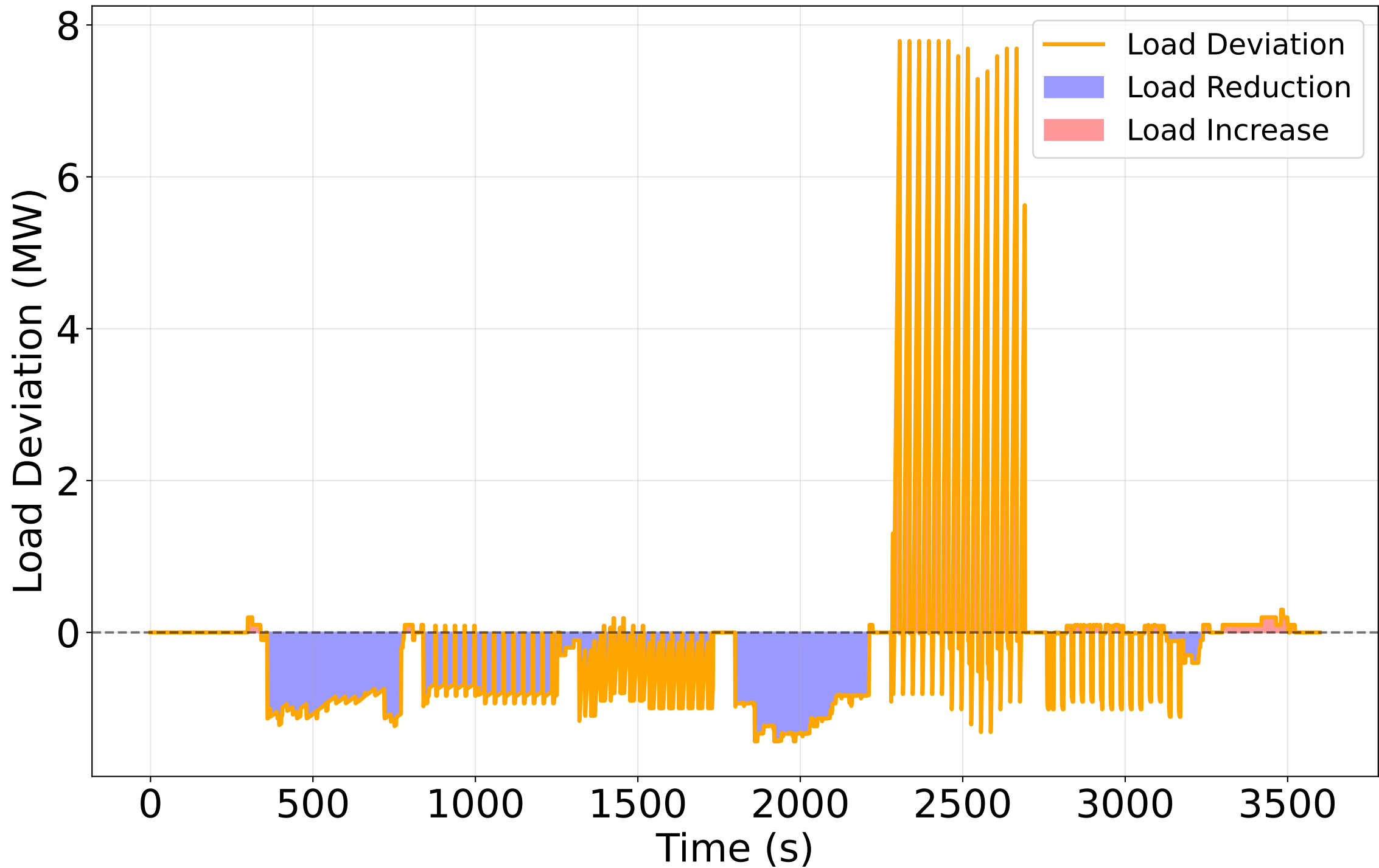
Attack-Induced Load Deviation
