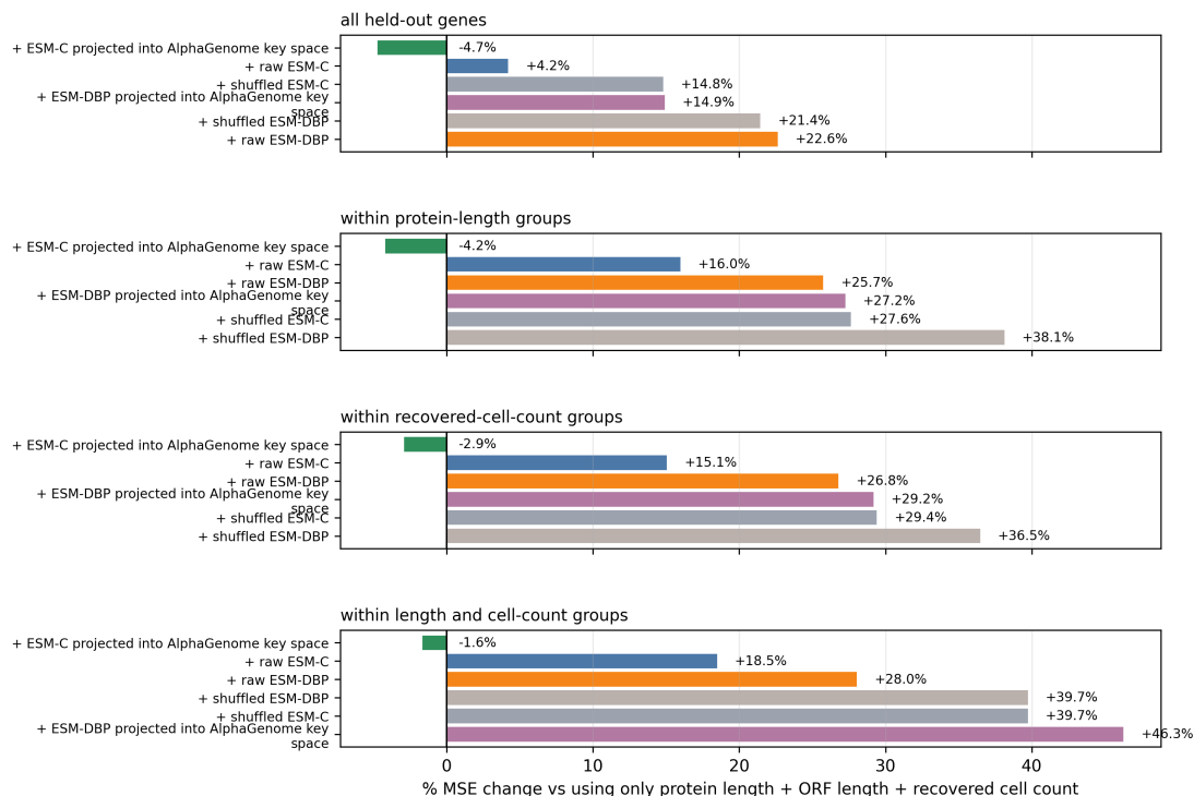
Figure 3: MSE change after adding sequence features to a model that already uses protein length, ORF length, and recovered cell count. ESM-C projected into ALPHA GENOME key space modestly improves in protein-length groups, recovered-cell-count groups, and joint length-plus-cell-count groups; ESM-DBP is worse in the same comparisons.
